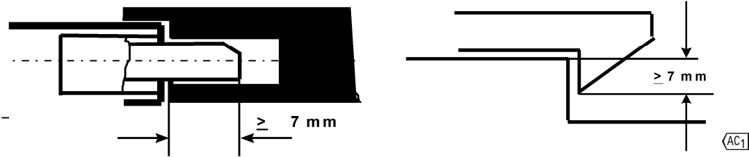
Figure 3 — Examples of locking elements
