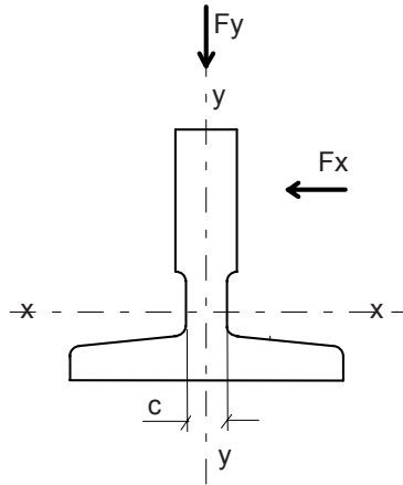
Figure G.1 : Axis of the guide rail
