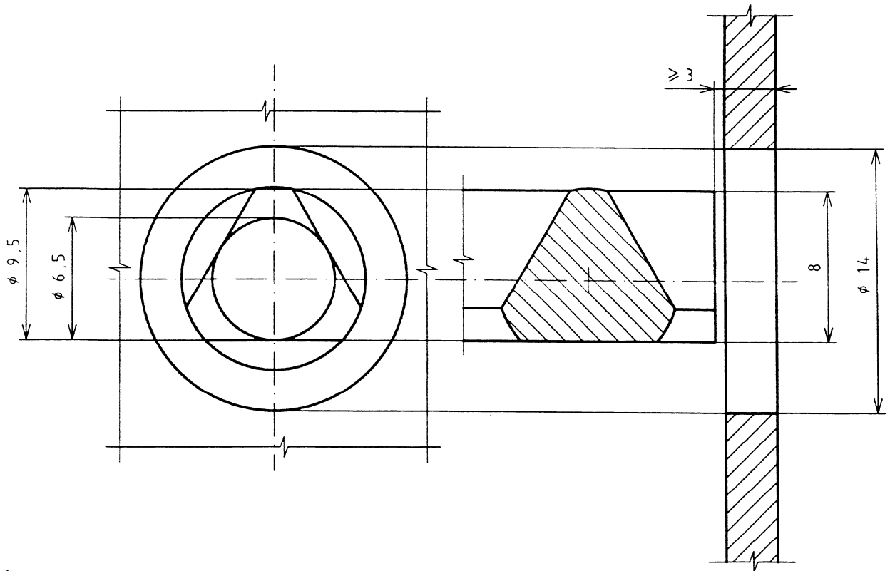
Figure B.1 : Unlocking triangle
