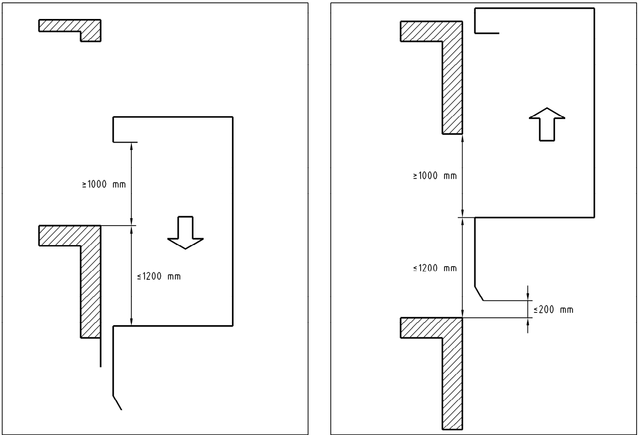
Figure 4 — Unintended car movement
