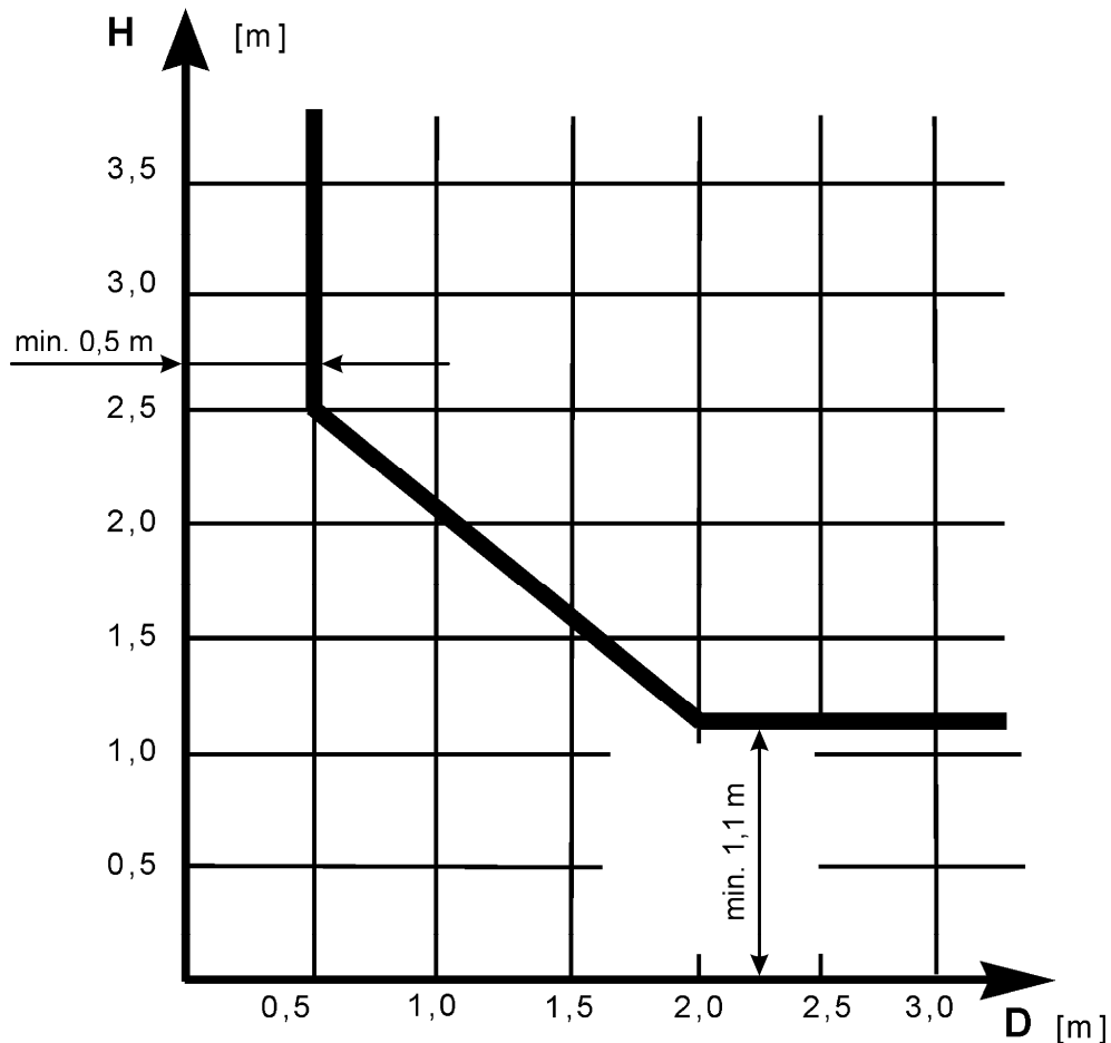
Figure 2 — Partially enclosed well – Distances
