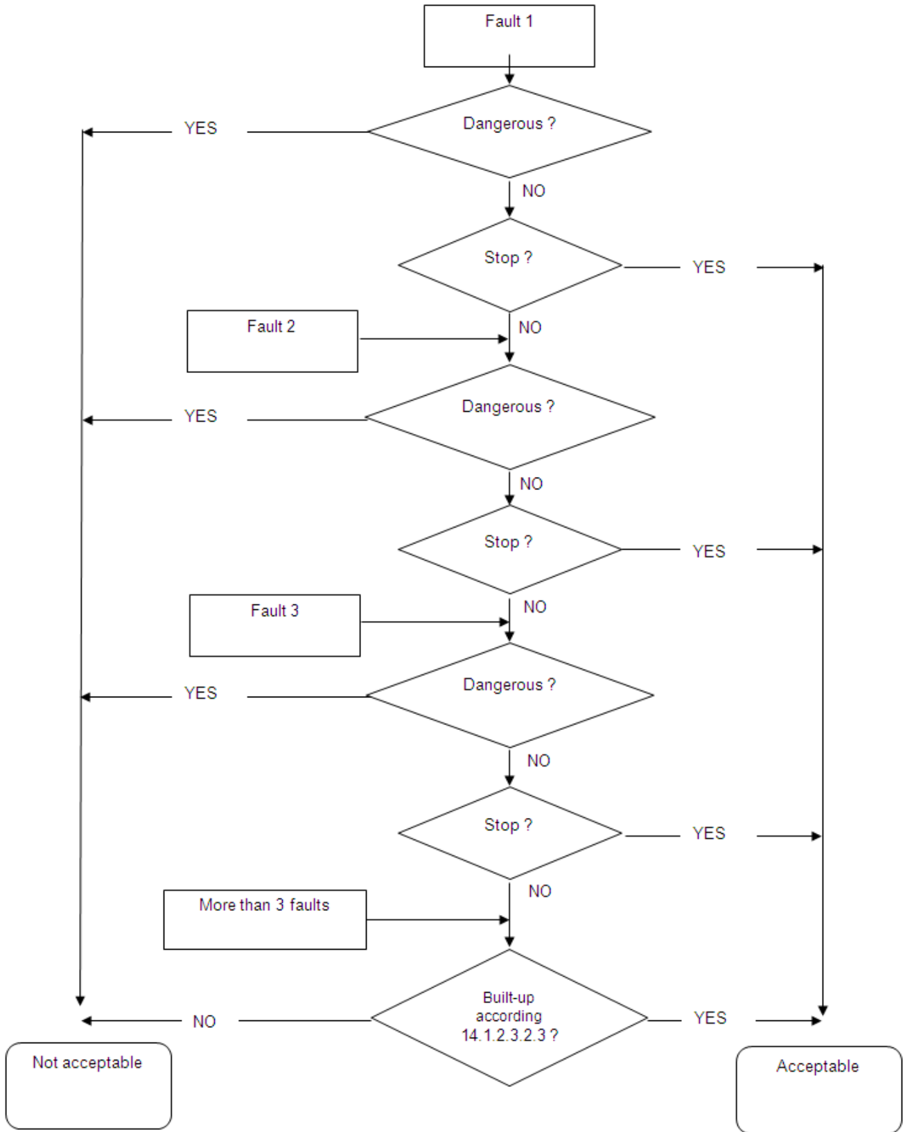
Figure 7 : Diagram for assessing safety circuits
