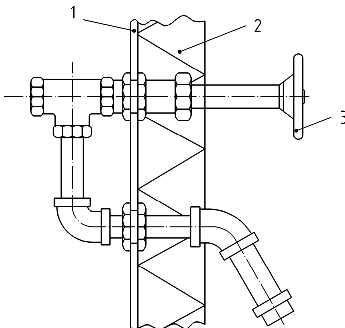
Figure 1 — Sampling probe with an outside stop-valve
