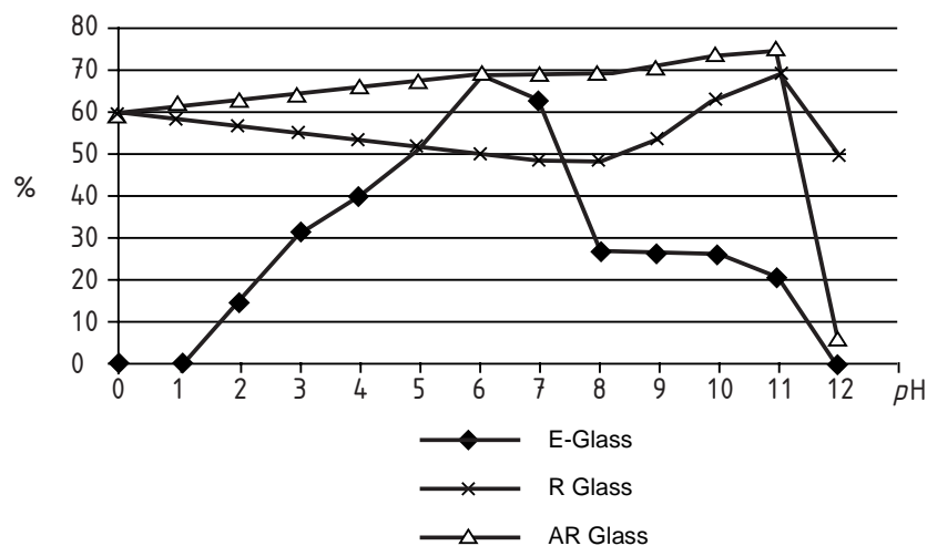
Figure A.1 - Retained tensile strength with pH
