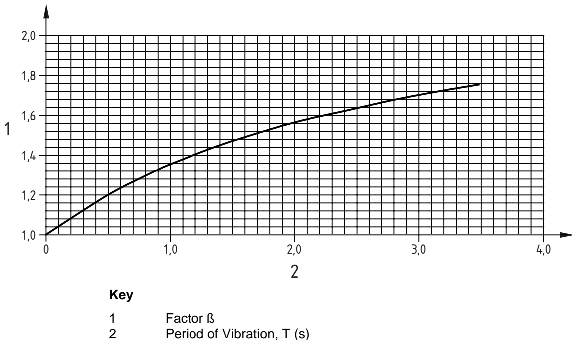
Figure B.1 — Coefficient \beta for the dynamic behaviour of fibre reinforced polymer composite columns
