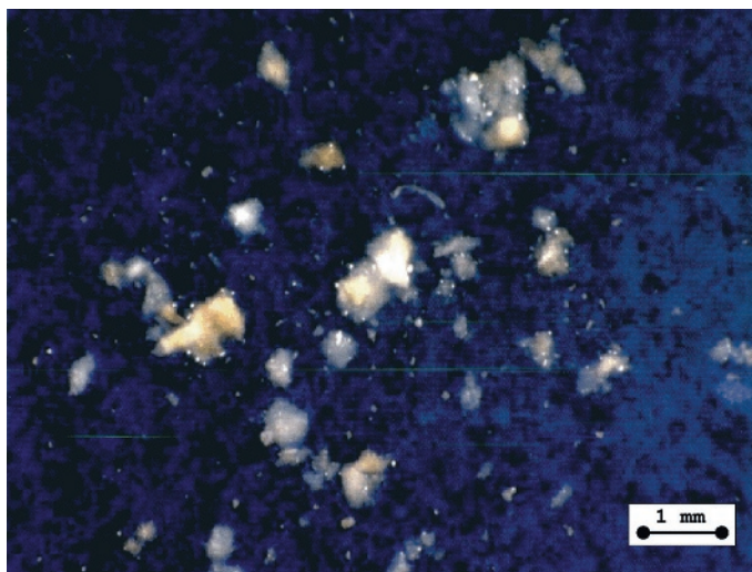
Figure 11 — Refractory clay particles in an enamel surface
