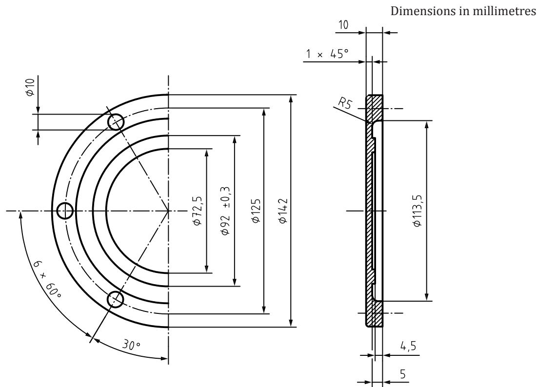
Figure 4 — Flange plate
