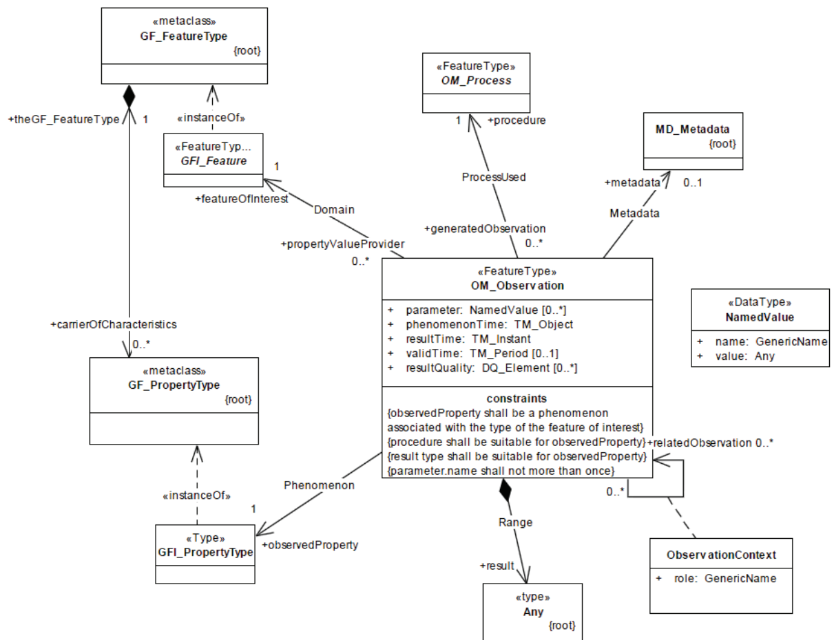
Figure C.1 — OM_Observation type (from ISO 19156)
