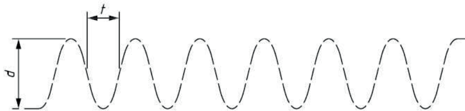
Figure 5 — Measurement of the grid in Figure 4 ; the spacing and depth of the grid are measured correctly
