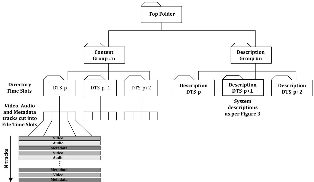
Figure 2 — Generic files organization
