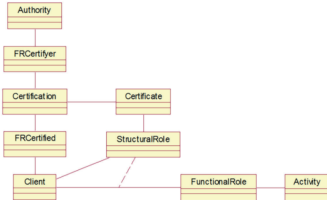
Figure 2 — Development of the role model
