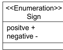
Figure C.8 — Example of <<Enumeration>>
