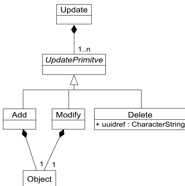
Figure C.23 — Update primitives
