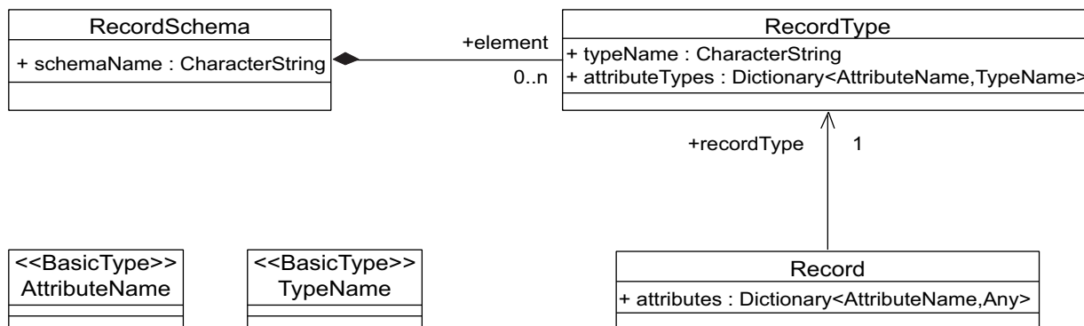
Figure C.11 — Record types
