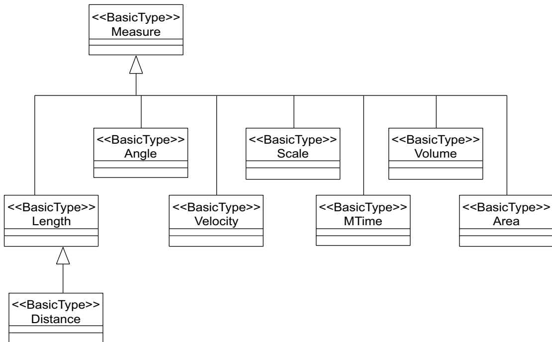
Figure C.7 — Measure types
