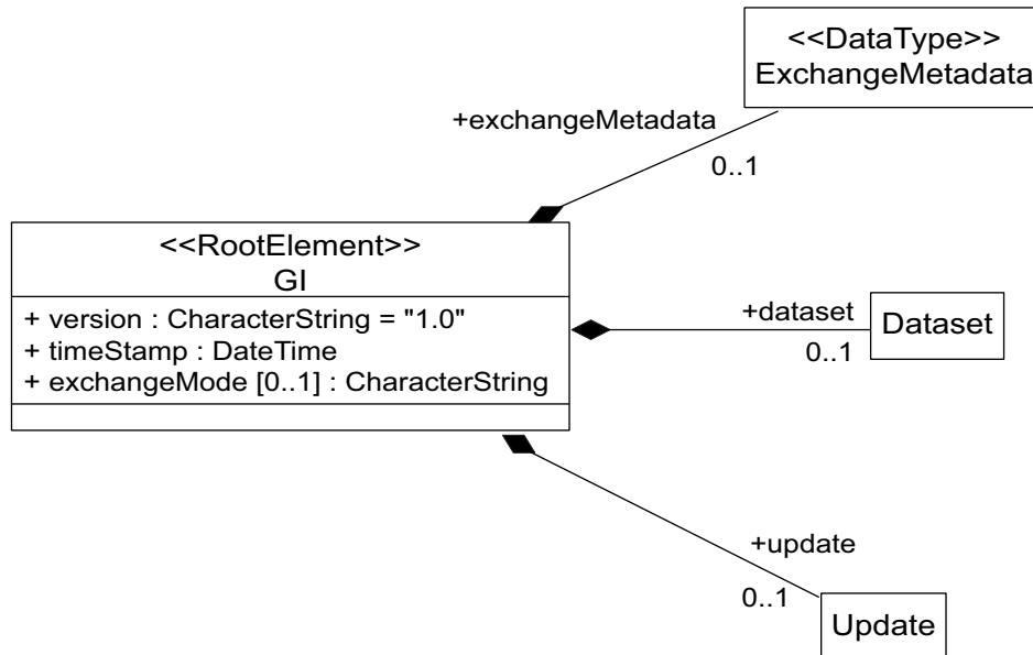
Figure C.20 — Document structure
