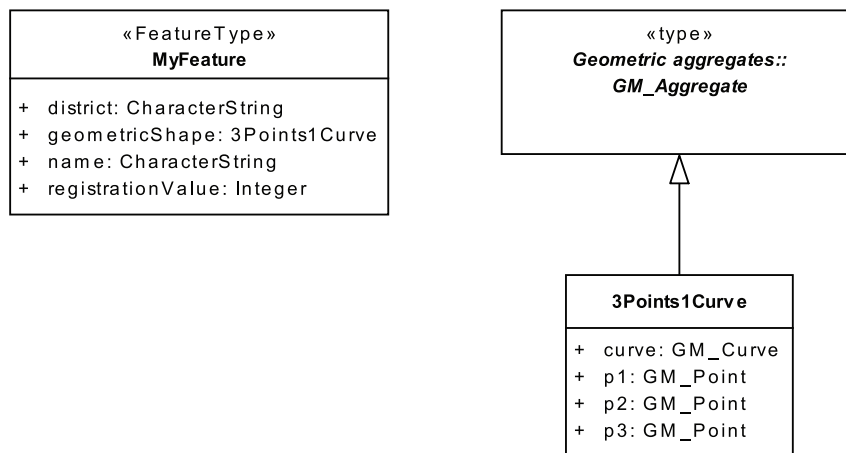
Figure 25 — Example of spatial aggregate defined in application schema
