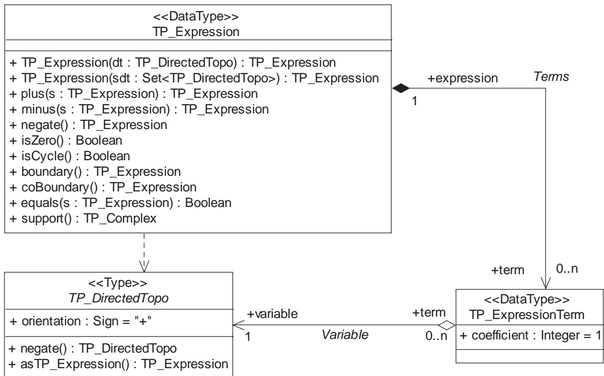
Figure 45 — TP_Expression
