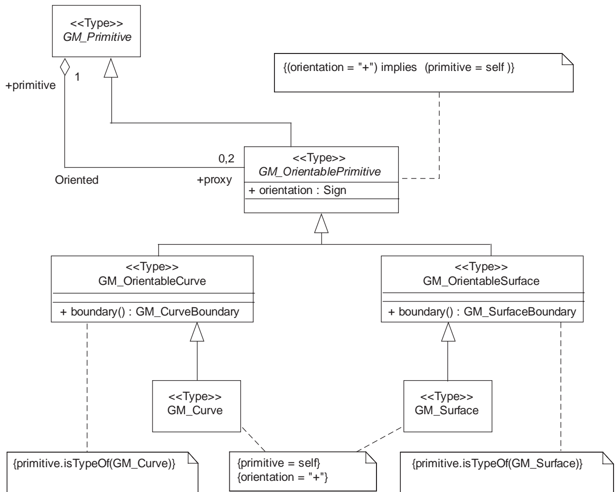
Figure 10 — GM_OrientablePrimitive
