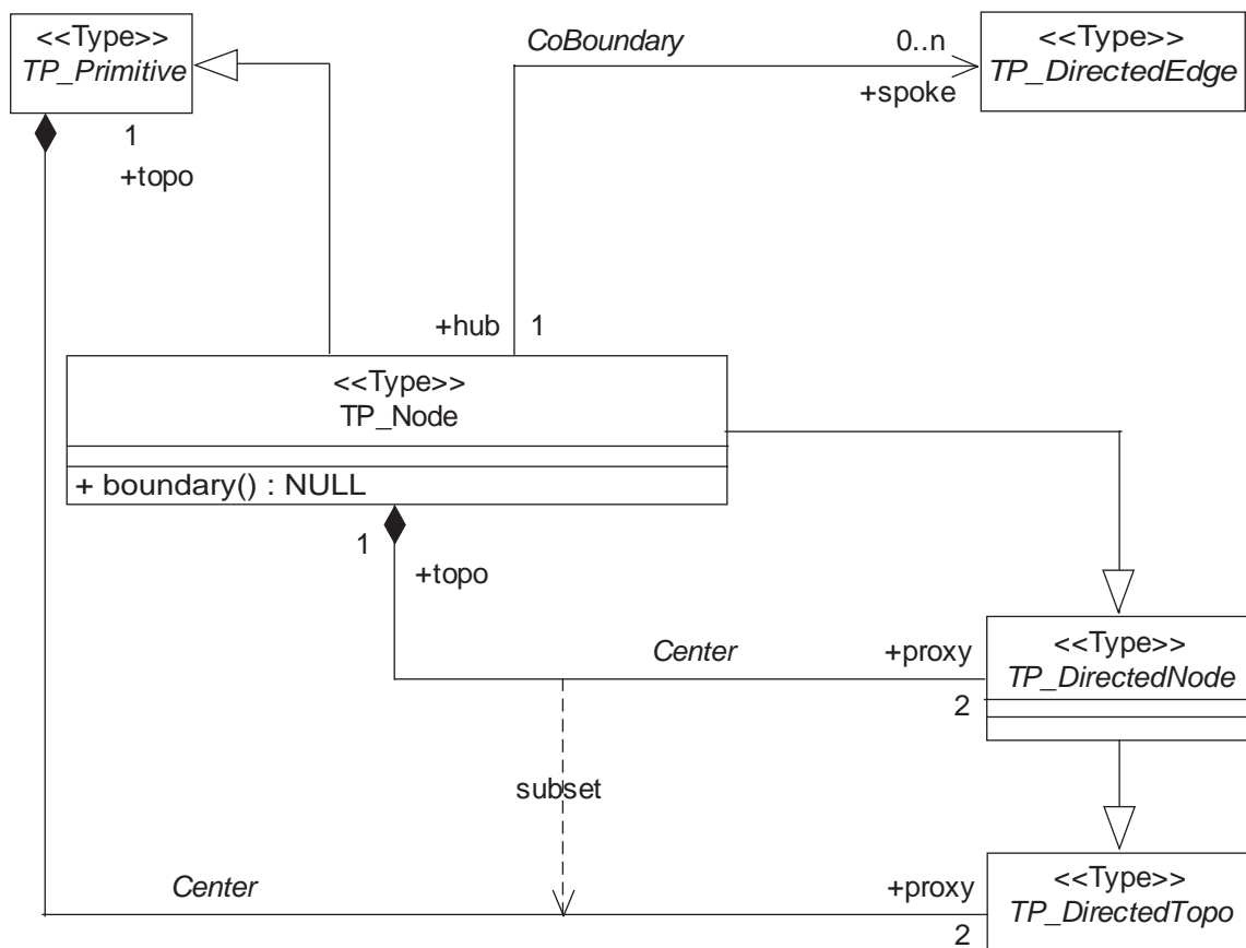
Figure 41 — TP_Node
