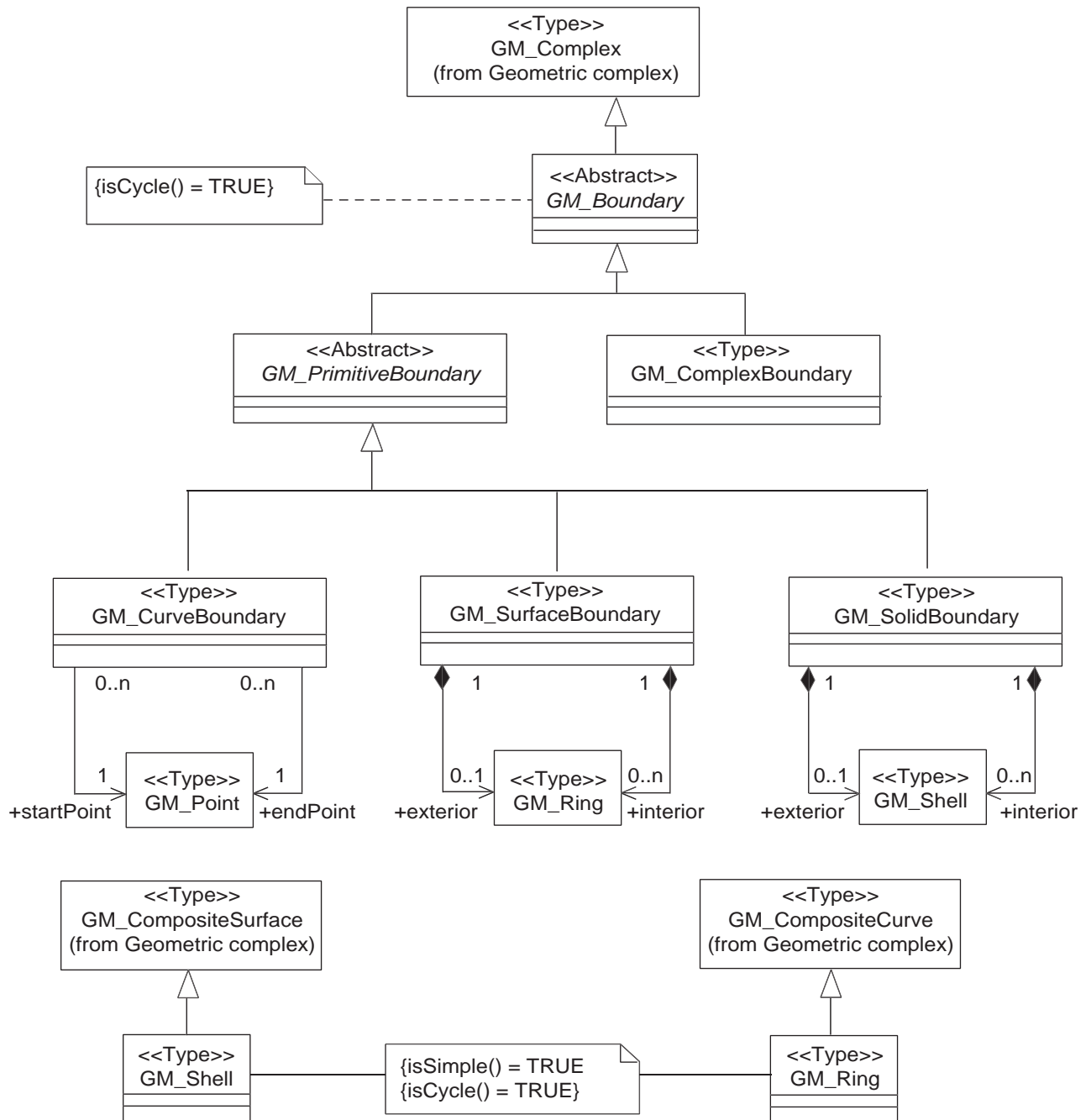
Figure 7 — GM_Boundary
