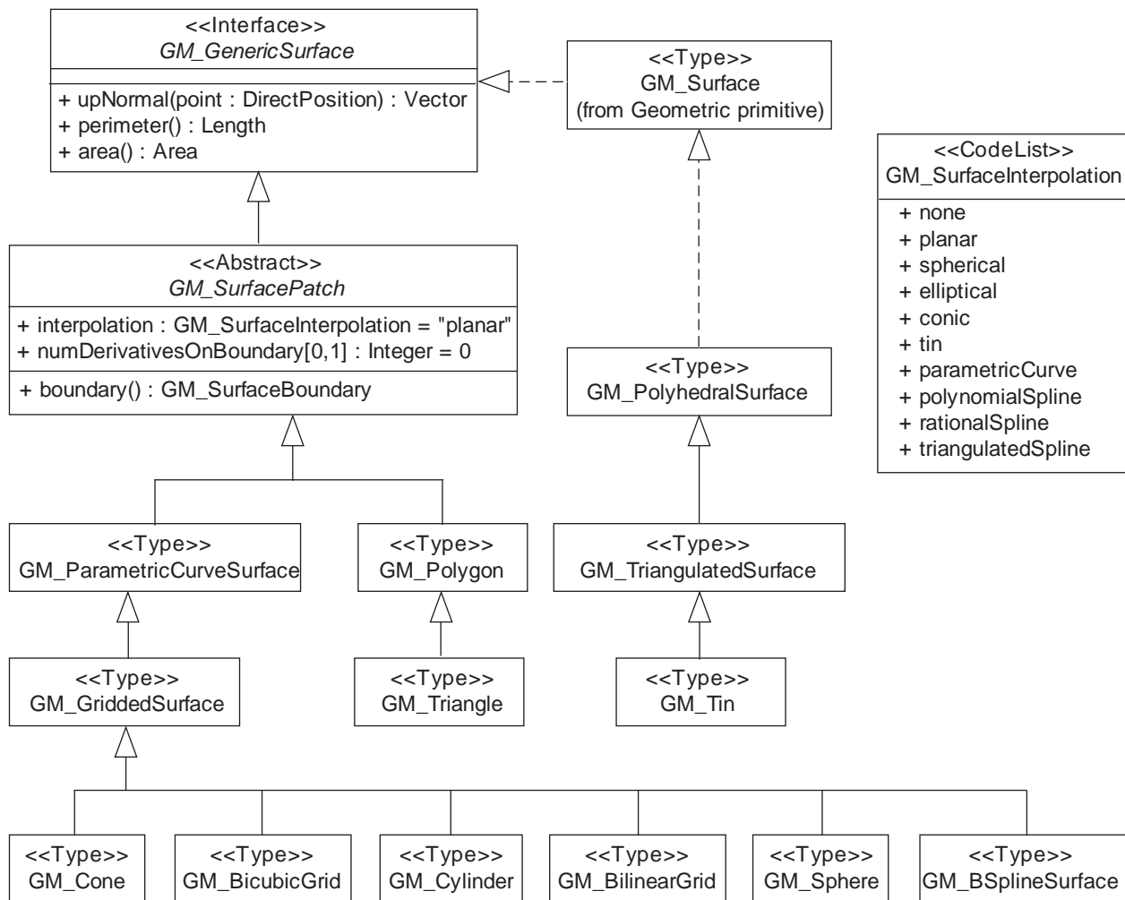
Figure 20 — Surface patches
