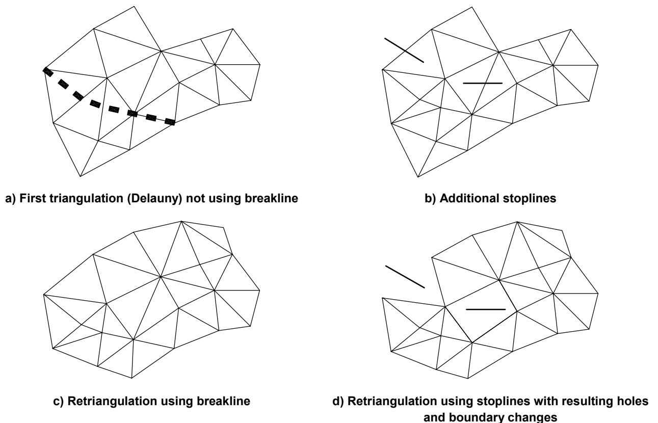
Figure 22 — TIN construction
