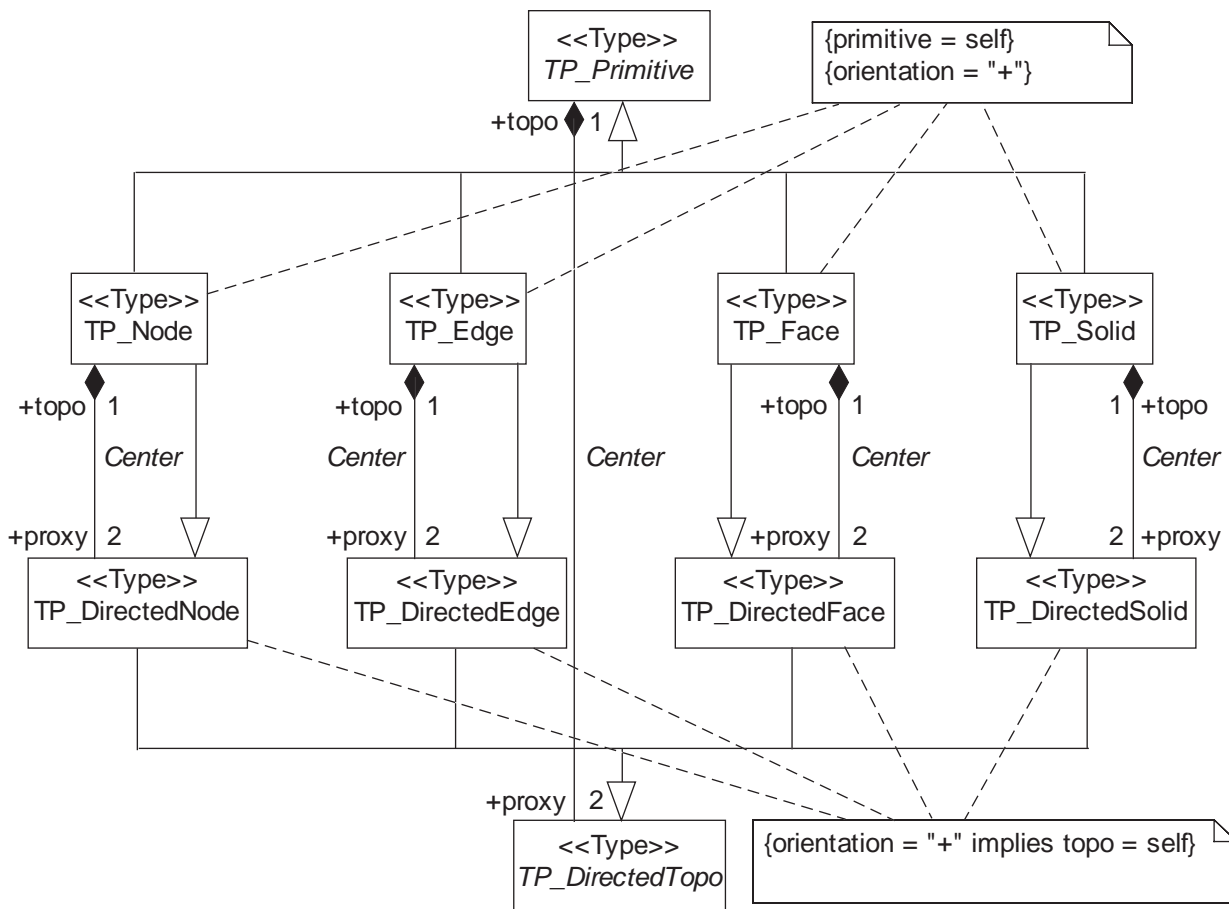
Figure 39 — TP_DirectedTopo subclasses
