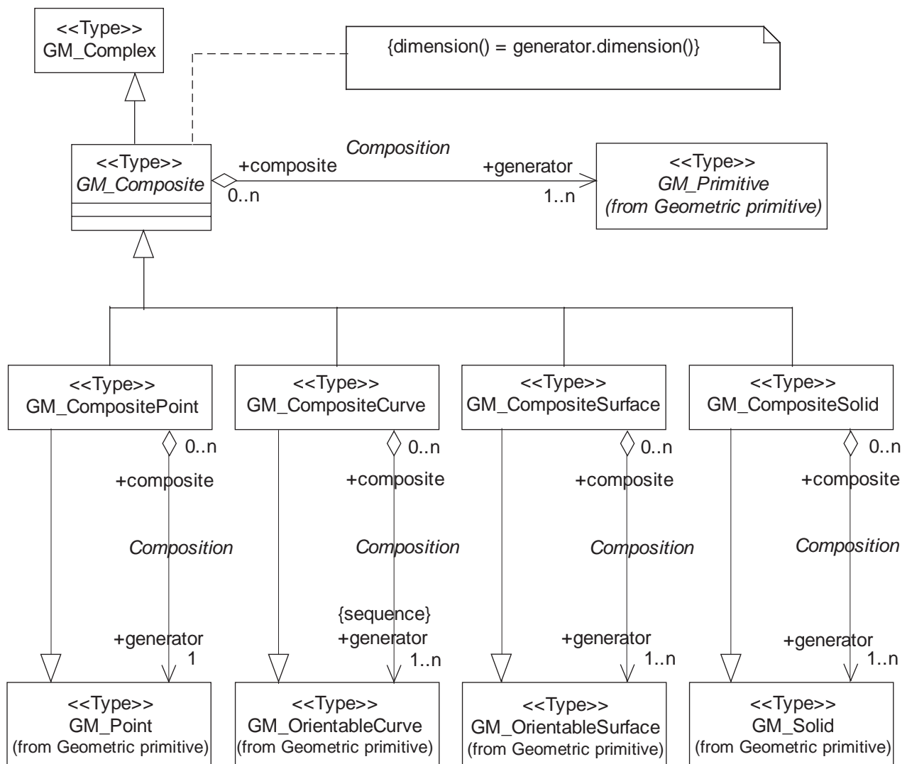
Figure 26 — GM_Composite
