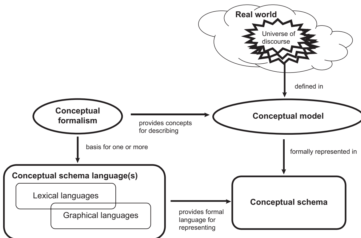
Figure E.1 — From reality to conceptual schema
