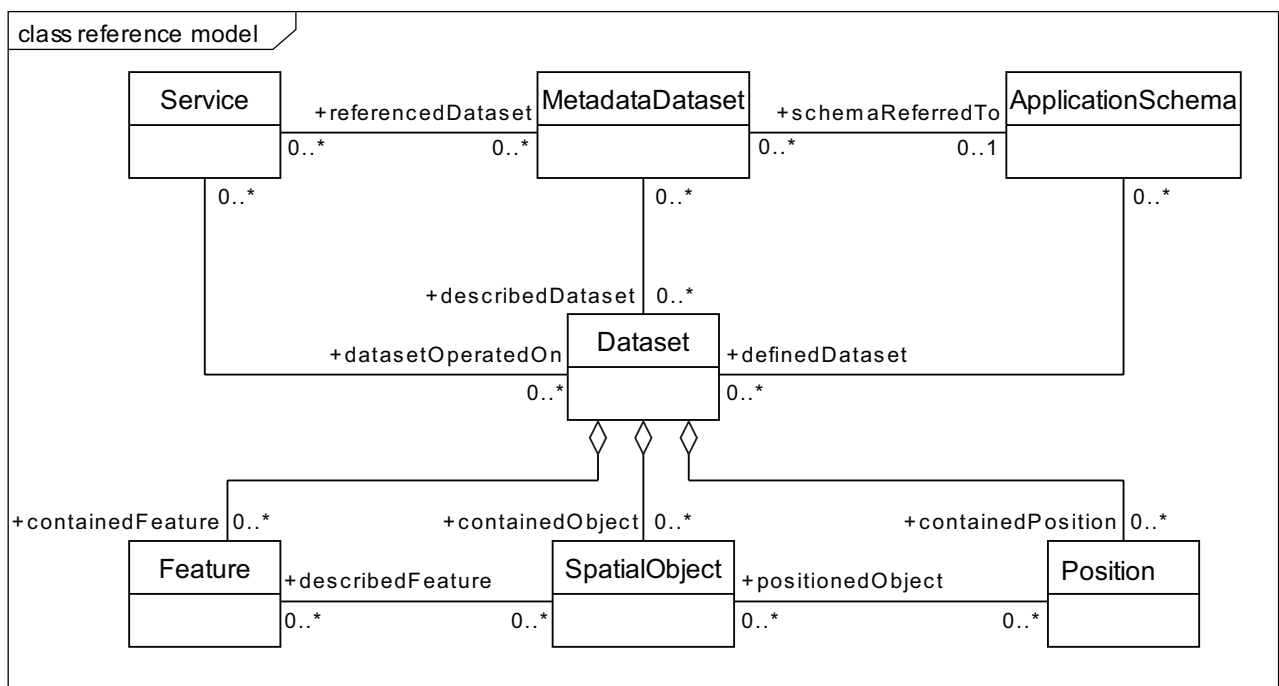
Figure 2 — High-level view of the domain of geographic information
