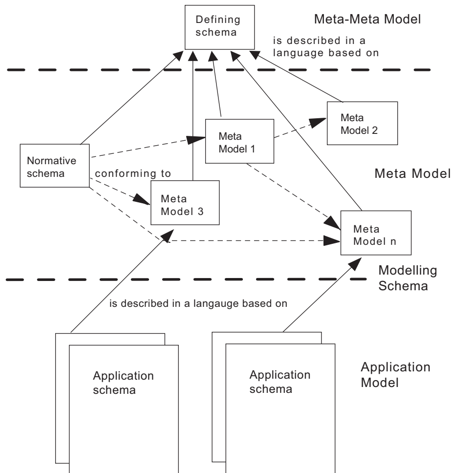
Figure G.1 — Conceptual Schema Modelling Facility schema architecture
