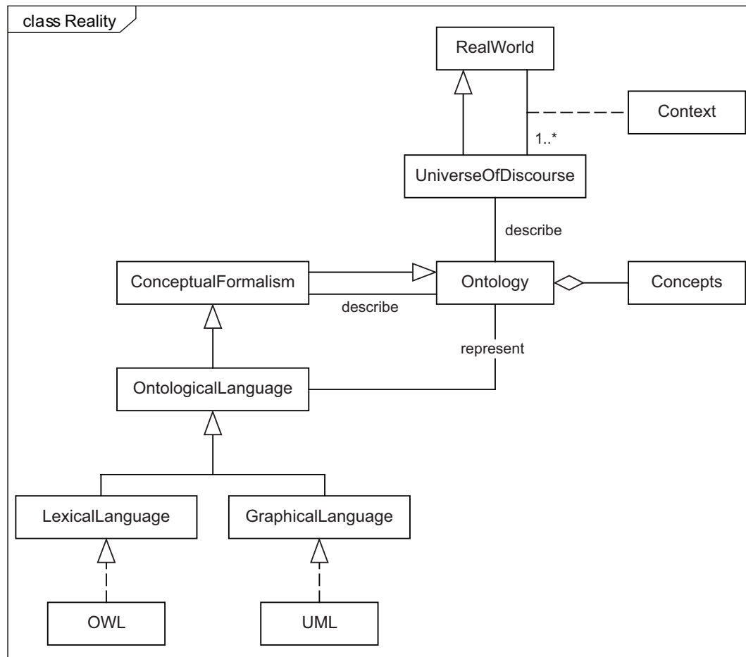
Figure E.2 — UML diagram depicting the abstraction of the real world
