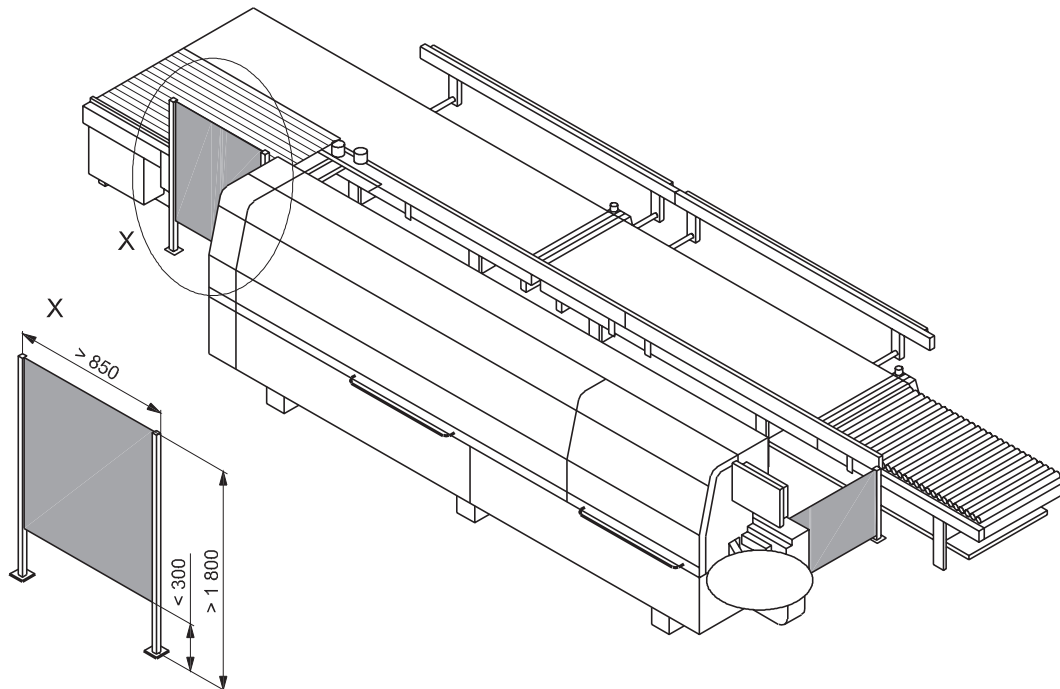
Figure 5 — Example of automatic panel returner
