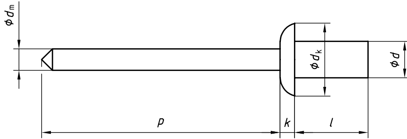
Figure 1 — Rivet dimensions
