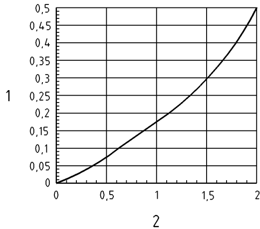
Figure C.2 - NPIP margin for mean piston/plunger speed
