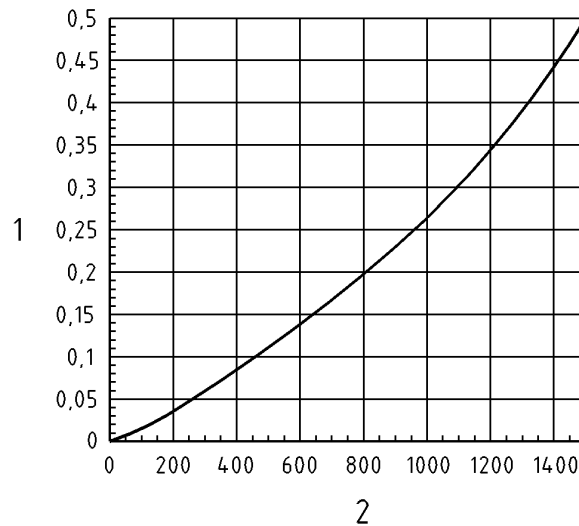
Figure C.1 NPIP margin for pump speed
