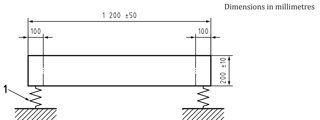
Figure A.1 — Concrete slab
