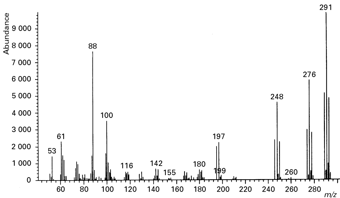
Figure D.4 — Mass spectrum of bromoxynil
