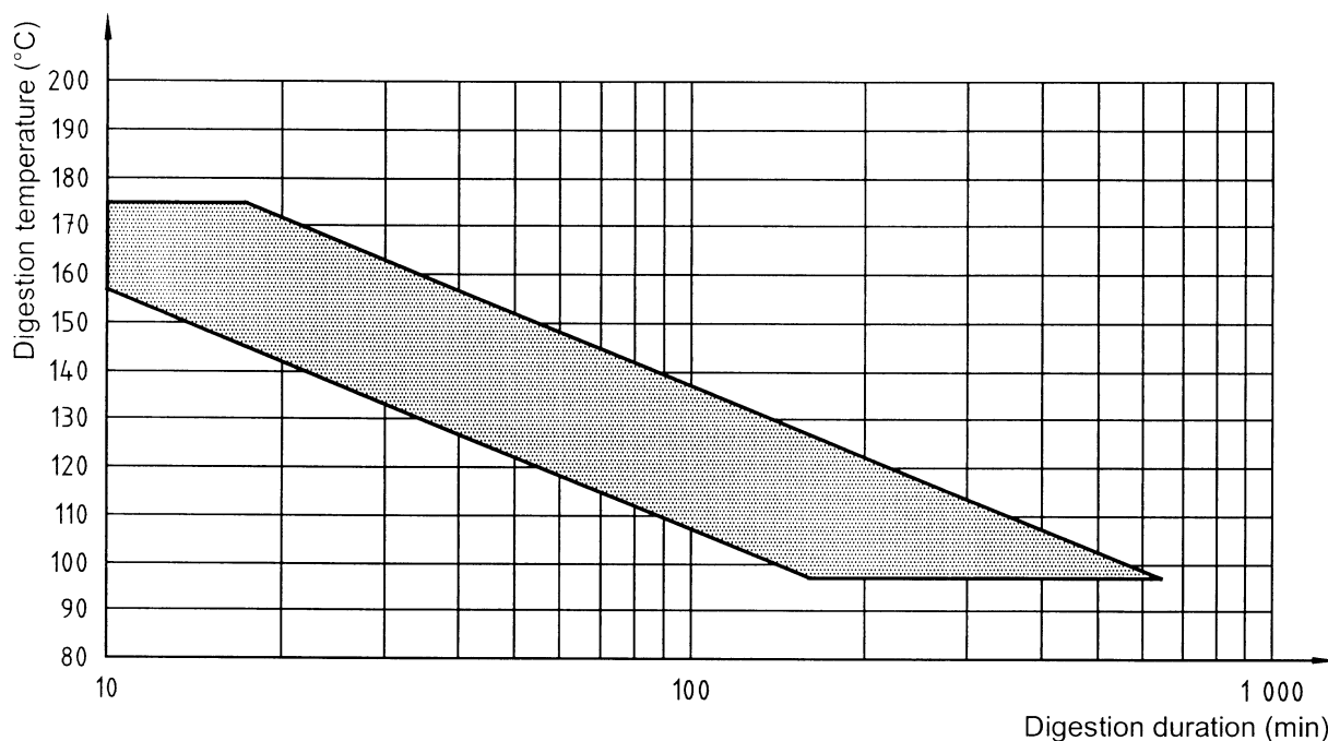
Figure 1 — Domain of permitted digestion temperature and duration
