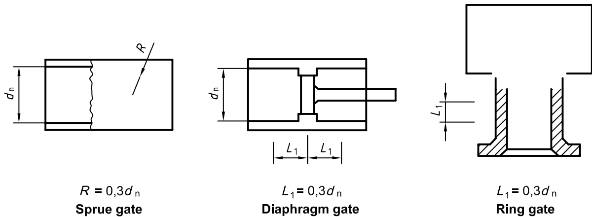
Figure B.5 — Injection gating areas
