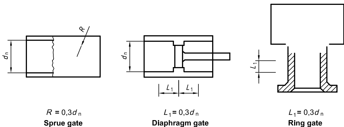
Figure C.7 — Injection gating areas
