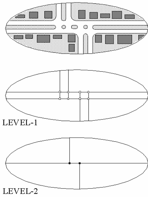
Figure F.14 — Further example of Level-2 formation of Intersections at crossings with traffic islands
