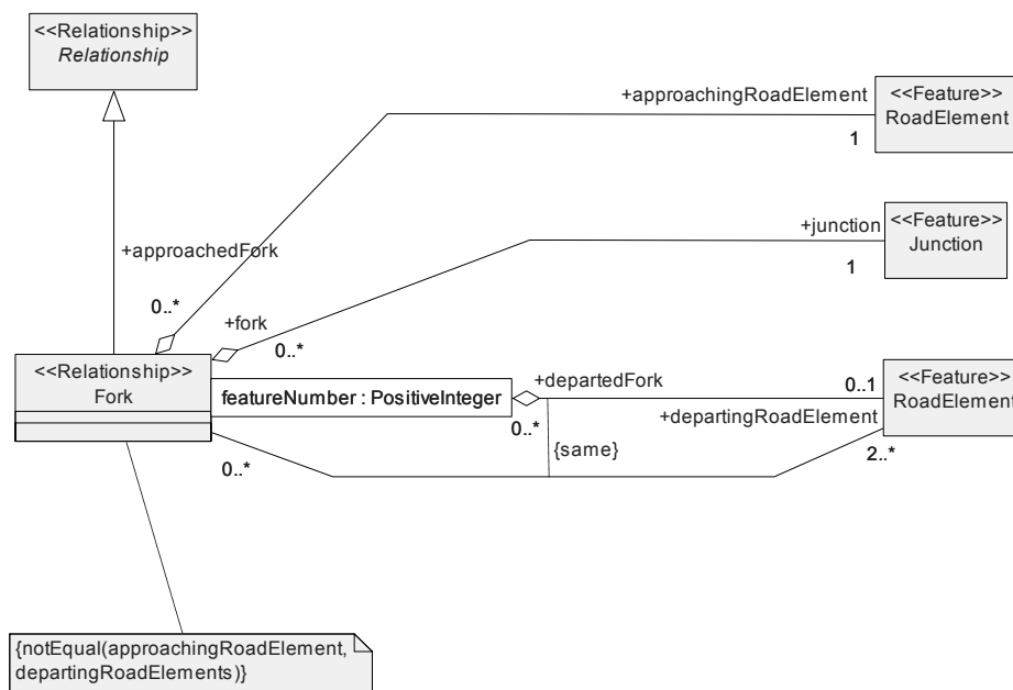
Figure 144 — The Conceptual Data Model for the Fork Relationship
