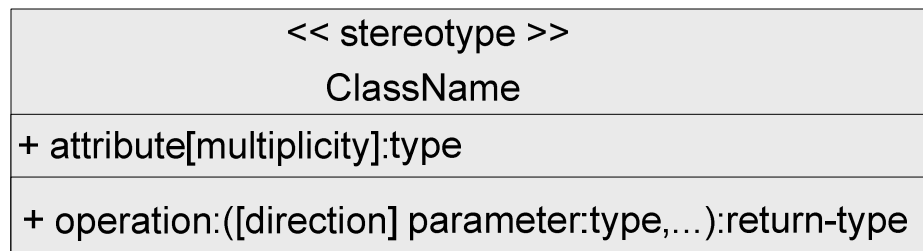
Figure 1 — Class with attributes and operations
