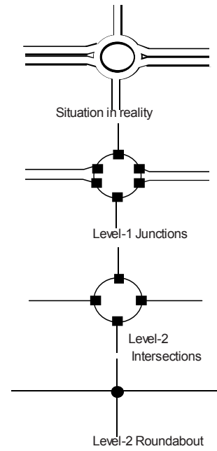
Figure F.15 — An example of Level-2 formation of roundabouts
