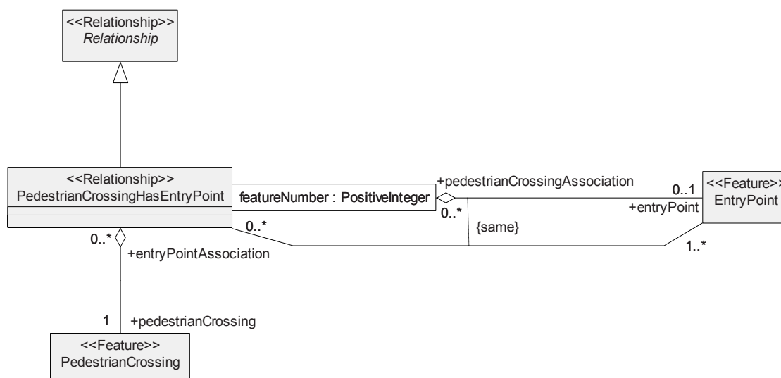
Figure 162 — The Conceptual Data Model for the Pedestrian Square Connected To Pedestrian Crossing Relationship
