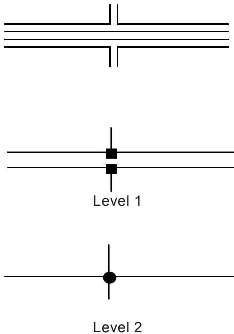
Figure F.8 — A crossing between two non-connected single carriageways and a multi carriageway
