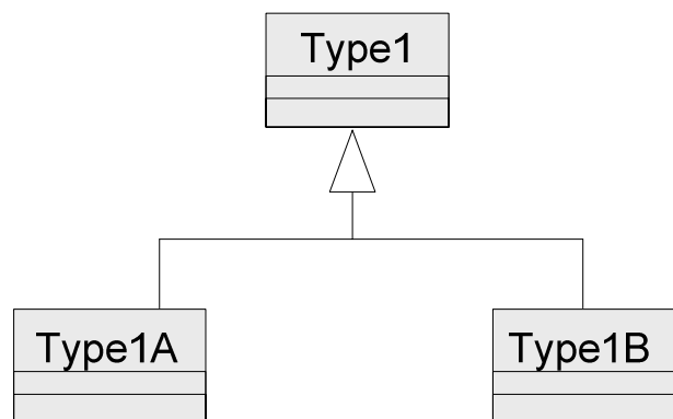
Figure 3 — Subclass hierarchy
