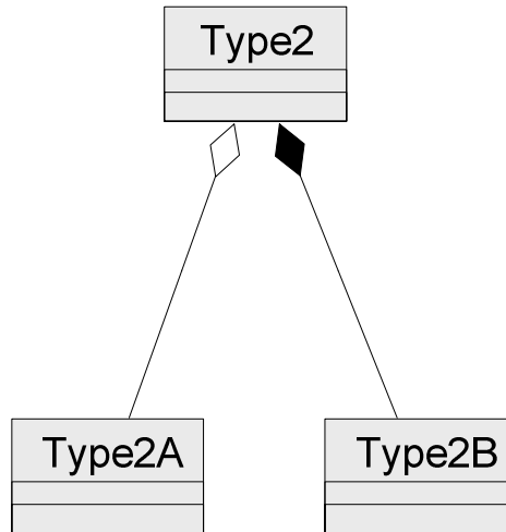
Figure 5 — Aggregation/composition associations
