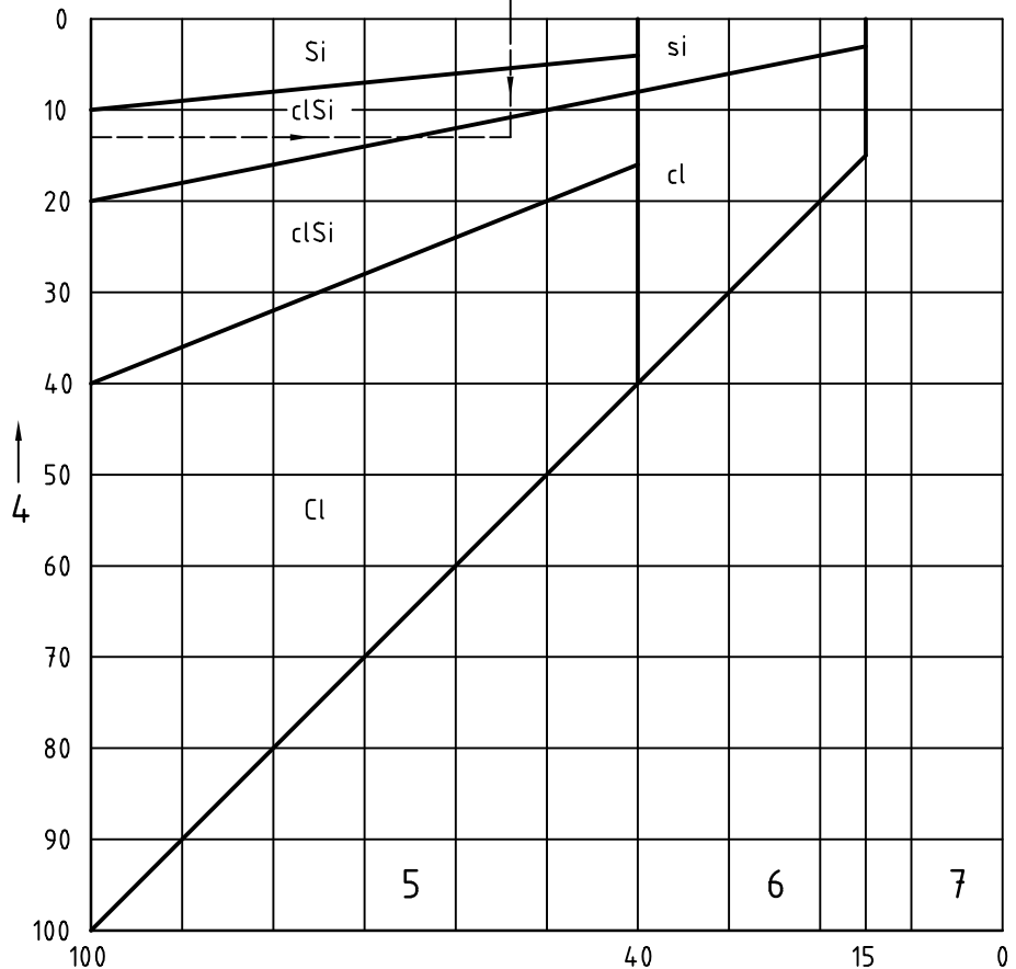
Figure B.1 — Classification of soils, based on grading alone
