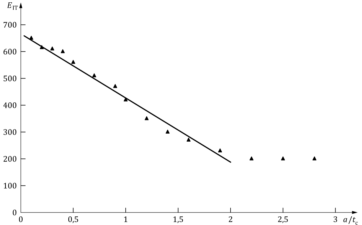
Figure 3 — Indentation modulus vs. normalized contact radius of hard brittle coating on a softer substrate — Schematically
