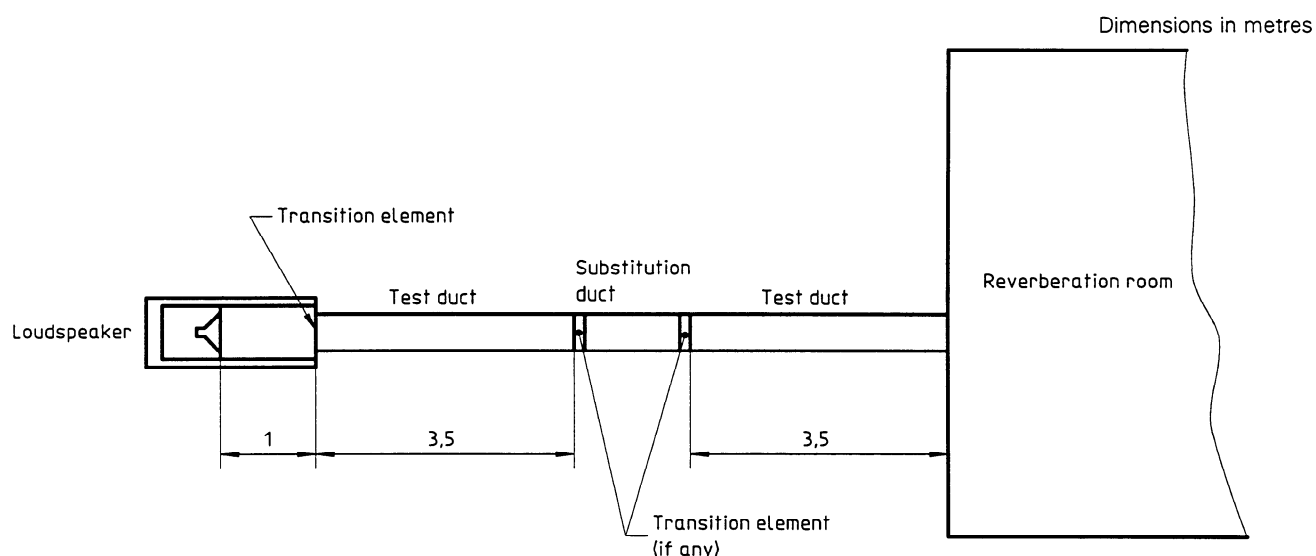
Figure 1 — Test facility
