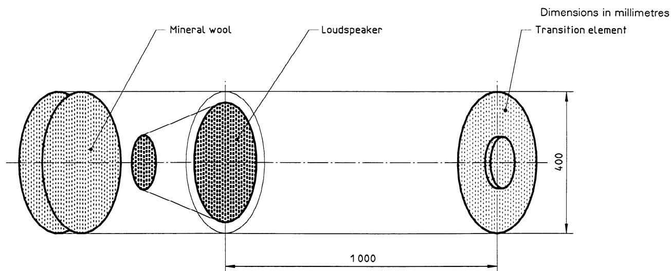
Figure 2 — Sound source
