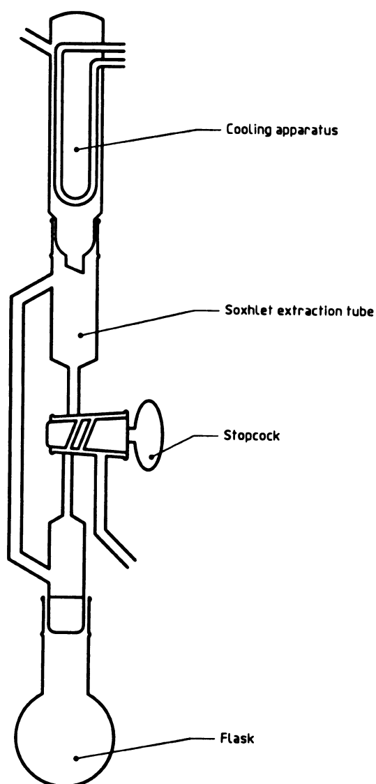
Figure 1 — Digestion apparatus
