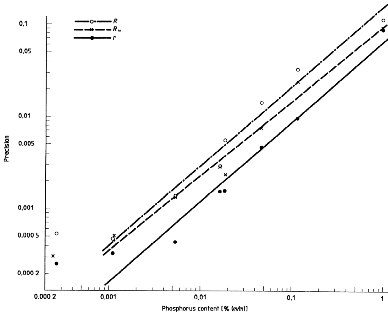
Figure B.1 — Logarithmic relationship between phosphorus content ( w_p ) and repeatability ( r ) or reproducibility ( R and R_w )
