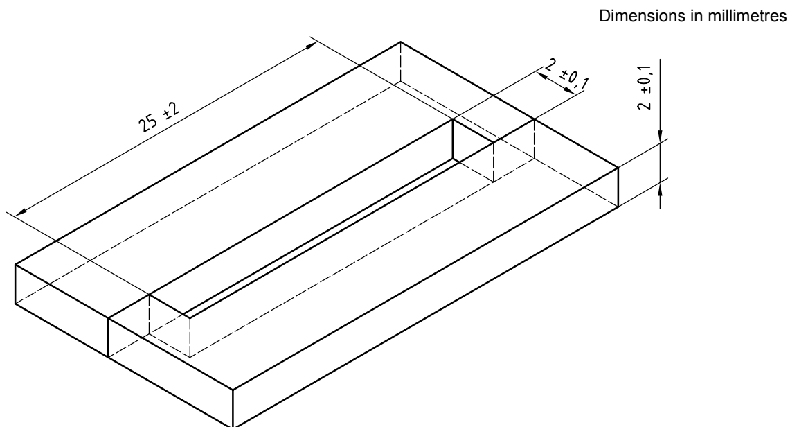
Figure 3 — Split mould for test specimens for the flexural test, made of stainless steel
