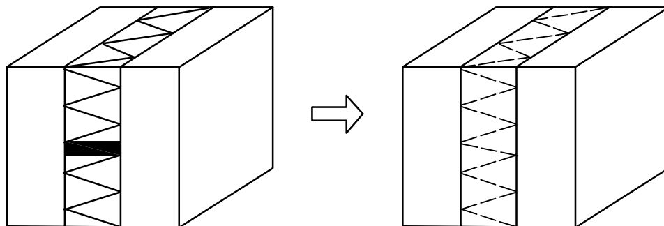
Figure 4 — Example of a minor point thermal bridge giving rise to three-dimensional heat flow, incorporated into a quasi-homogeneous layer
