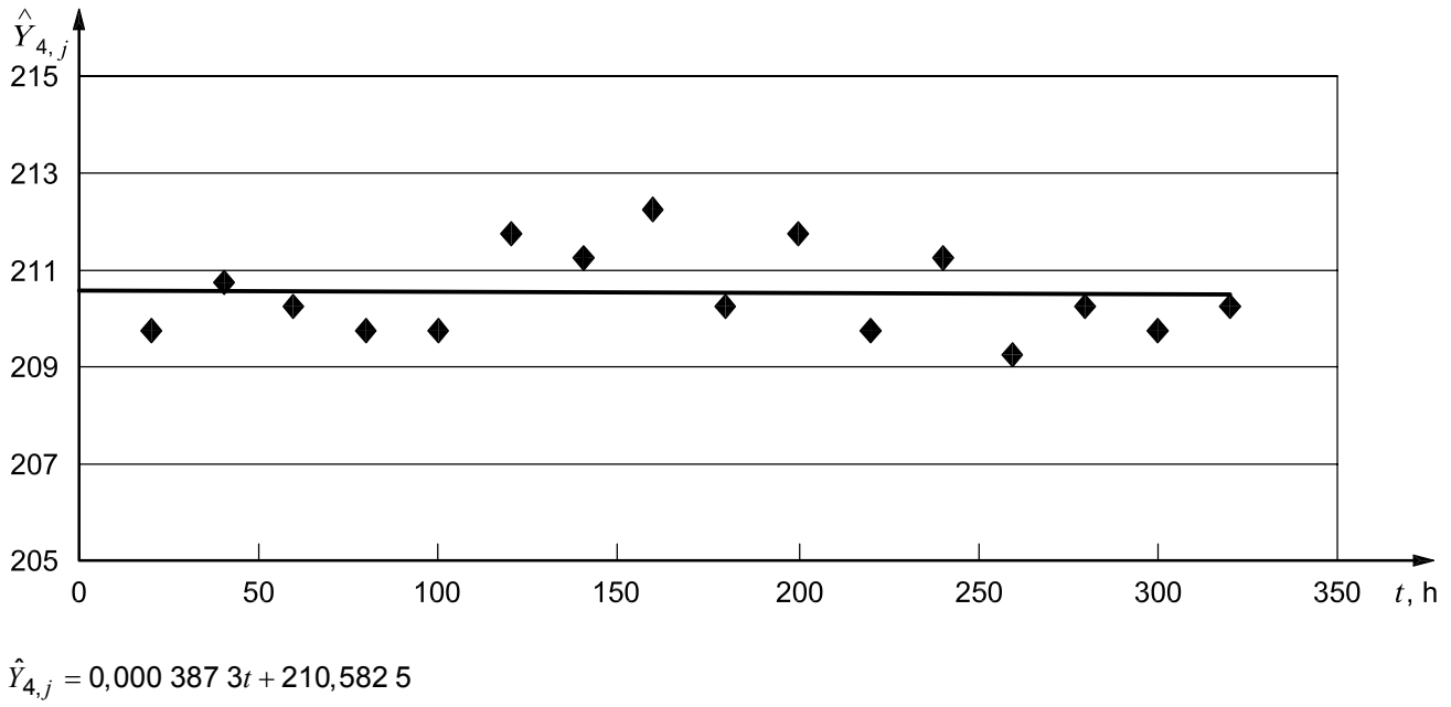
Figure A.3 — Result of drift test at concentration C_4
