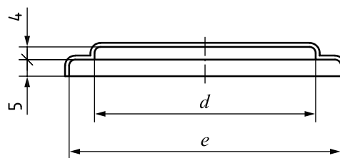
d) Lid with rim to fit outside dish (see Note to 6.4 for use of this assembly)
