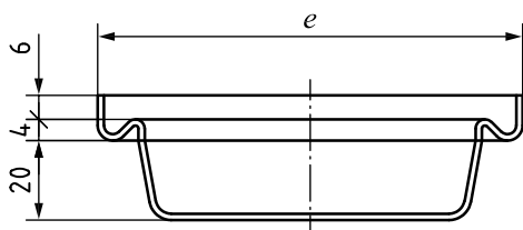
e) Deep dish
