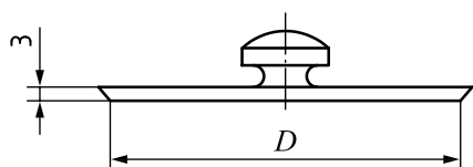
c) Cover template
