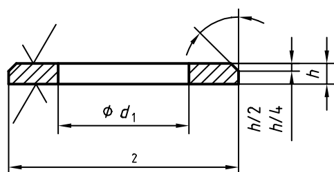
Figure 1 — Dimensions
