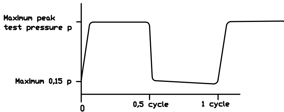
Figure F.1 — Pressure impulse cycle
