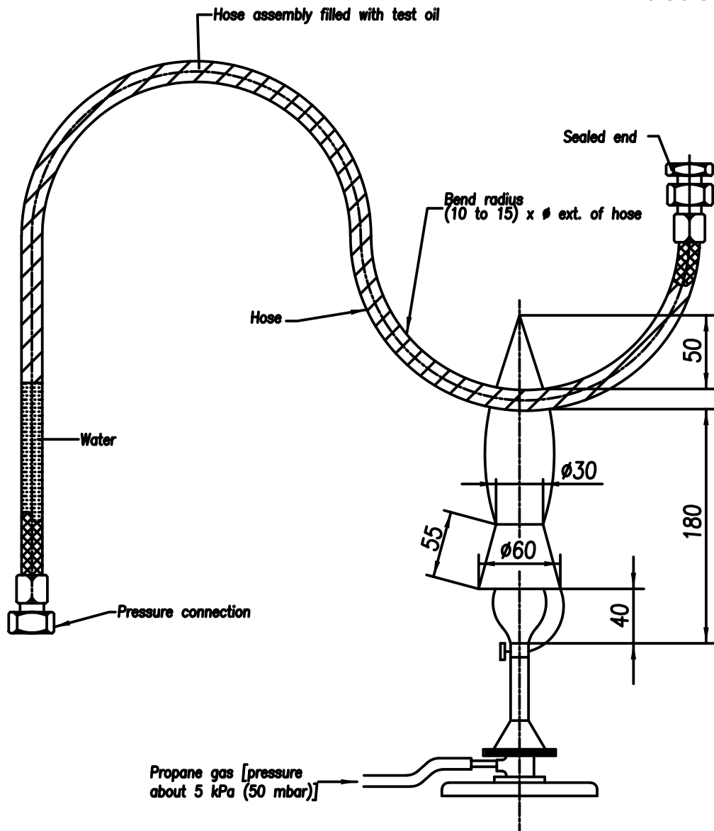
Figure E.1 — Arrangement for flammability test
