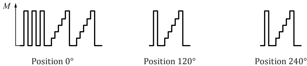
Figure C.2 — Examples of preloading and sequences for torque measurement devices with hexagon drive (minimum of four steps)
