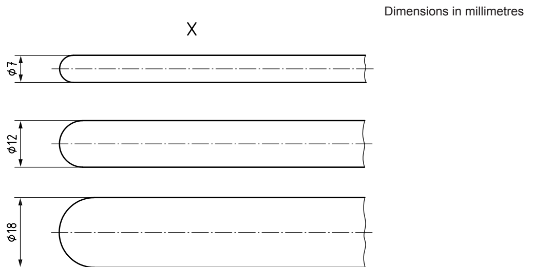
Figure 8 — Test probe
