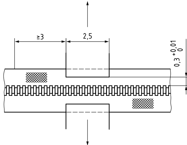
Figure 6 — Stretching to determine the maximum lateral strength
