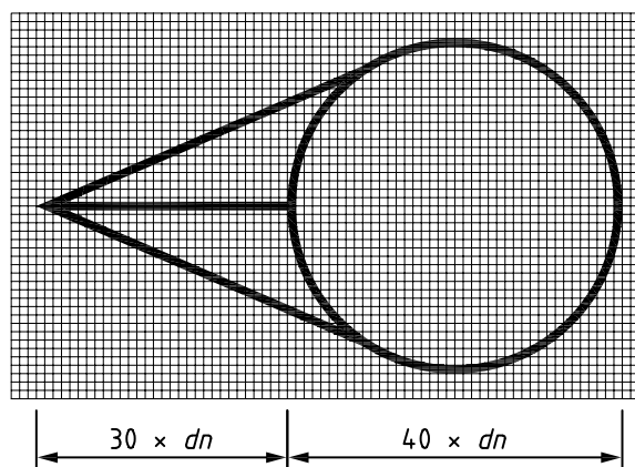
Figure F.1 — Moveable target frame
