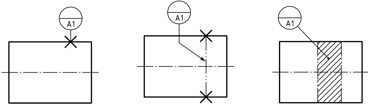
Figure 12 — Indicator for single datum target point
