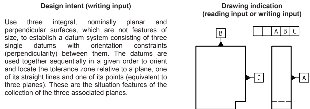
Figure C.35 — Three perpendicular planes — Input for reading (drawing indication) and for writing (design intent)
