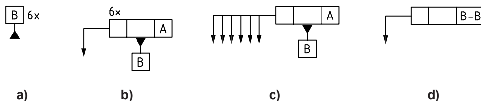
Figure 32 — Examples of complementary indication
