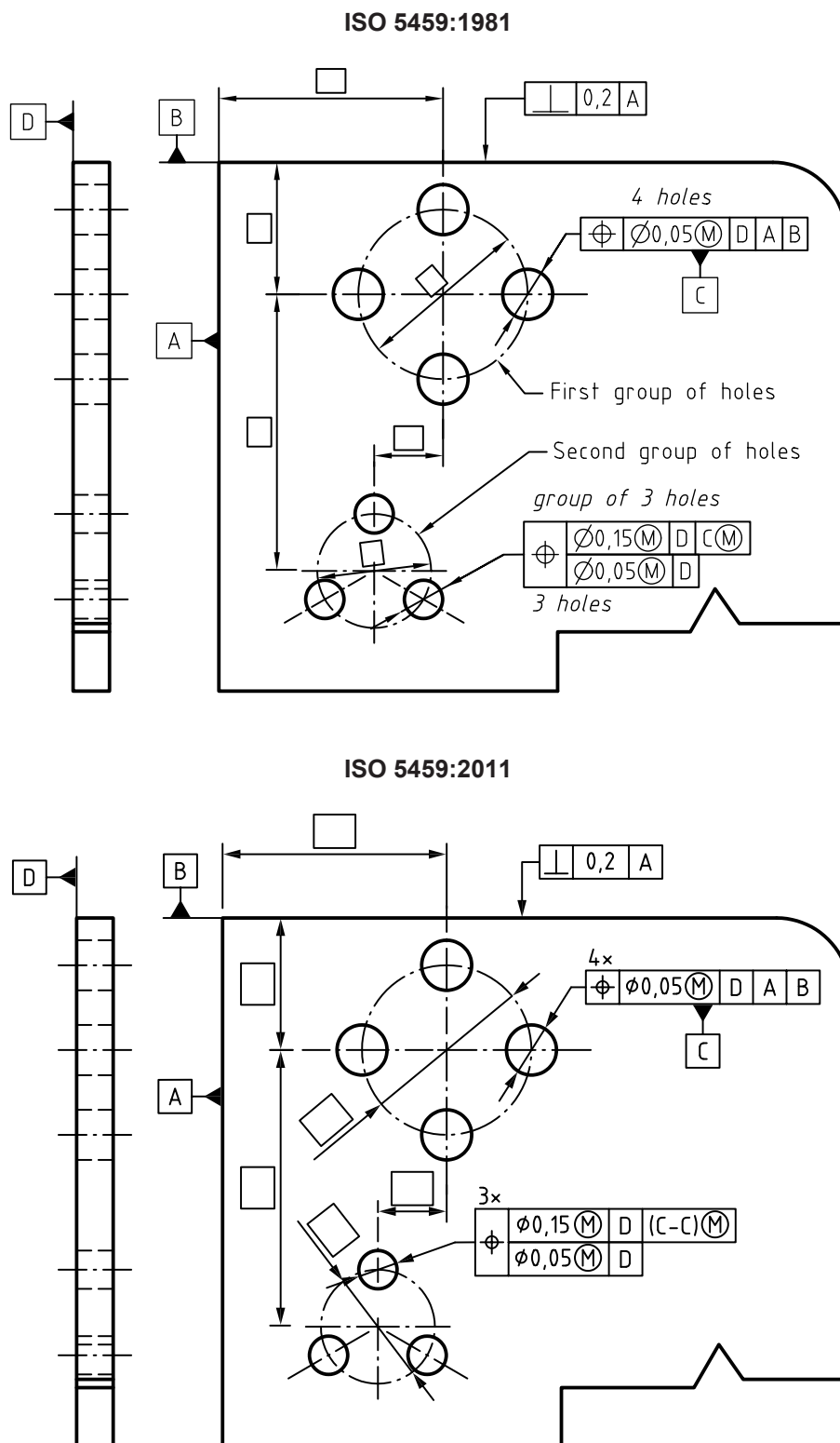
Figure D.3 — Indication of a common datum
