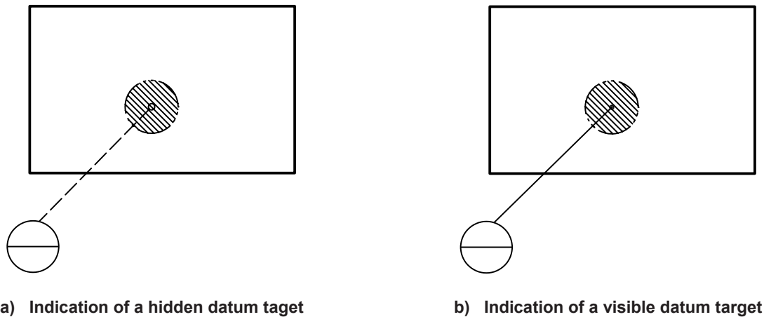
Figure 15 — Example of indication of datum target
