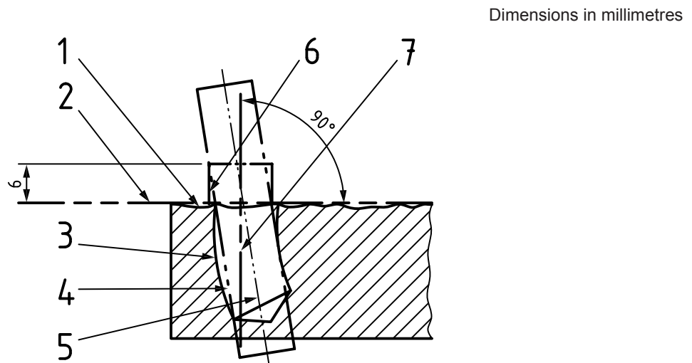
Figure 39 — Example of application of modifier \textcircled{P} on the secondary datum
