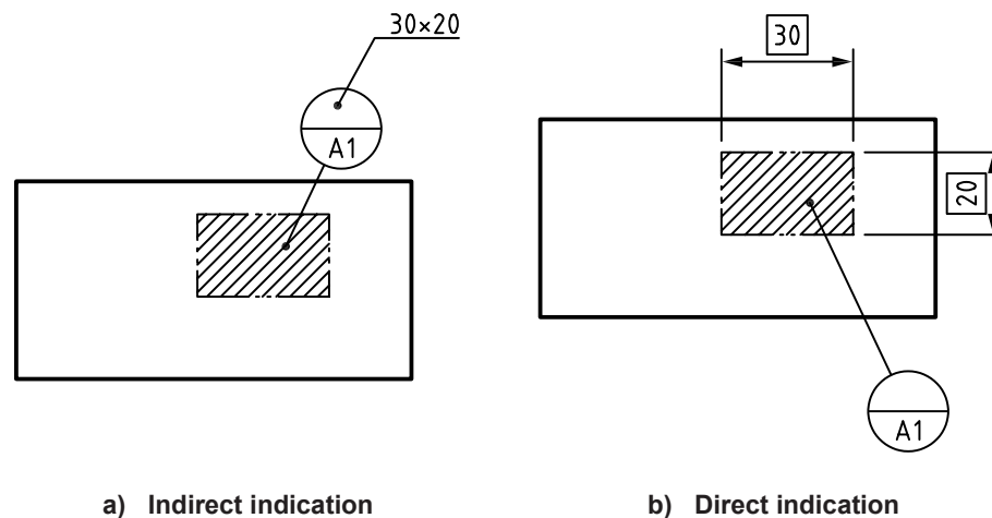
Figure 25 — Indication of dimensions of a rectangular area
