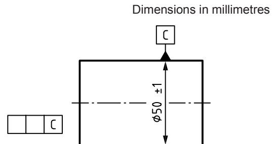
Figure C.3 — Cylinder — Input for reading (drawing indication) and for writing (design intent)
