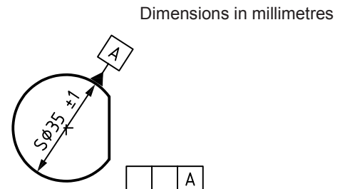
Figure C.7 — Sphere — Input for reading (drawing indication) and for writing (design intent)
