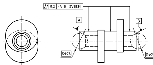
Figure 29 — Example of datum system in which the datum target indication is omitted
