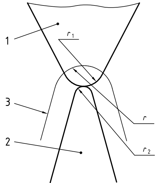
The output profile essentially represents the stylus tip shape if the radius and apex angle of the razor blade are much finer
