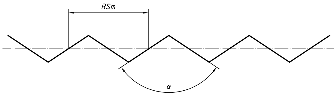
Figure 3 — Type B2 grooves (sensitive groove pattern)
