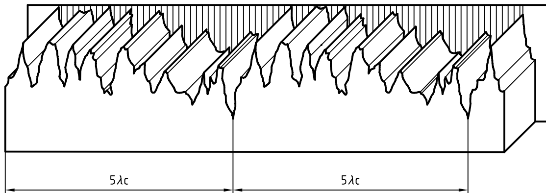
Figure 9 — Type D1 grooves (profile repetition at 5\lambda_c intervals)
