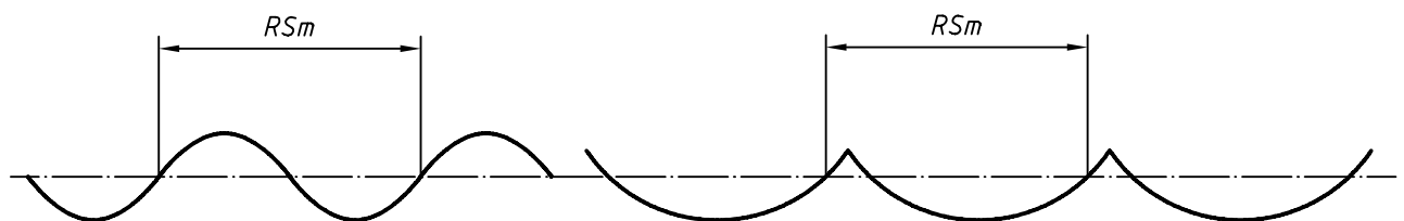
Figure 4 — Type B2 grooves (insensitive groove pattern)
