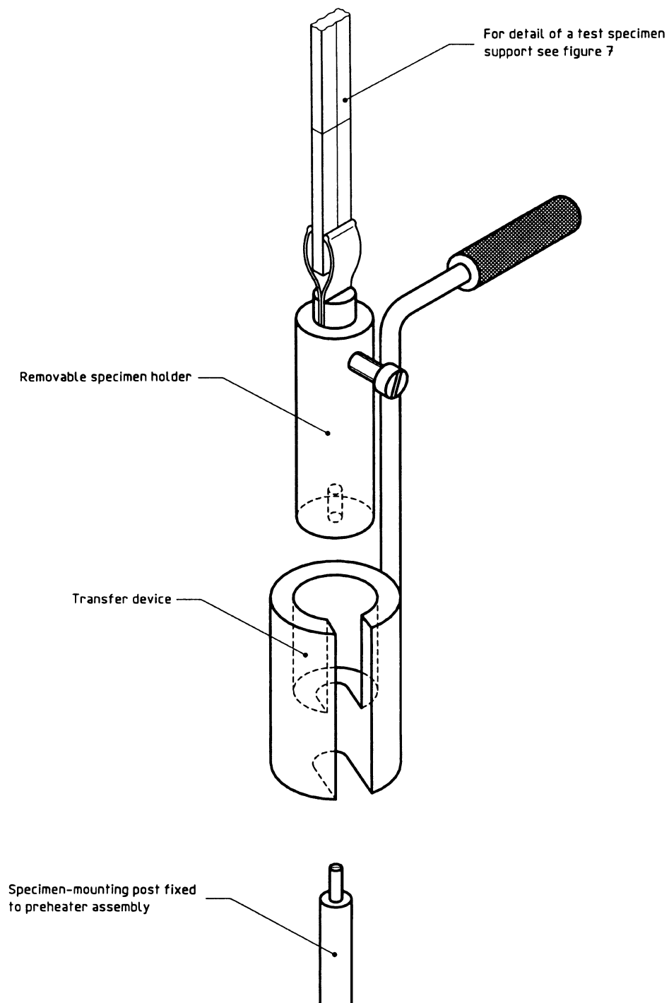
Figure 6 — Diagram of typical specimen-holder transfer tool
