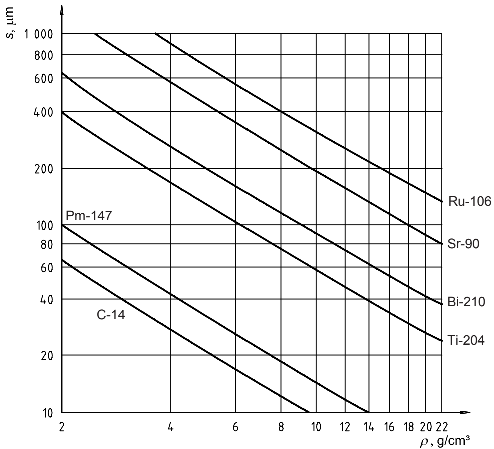
Figure A.1 — Saturation thickness, s , as a function of density, \rho , for different isotopes
