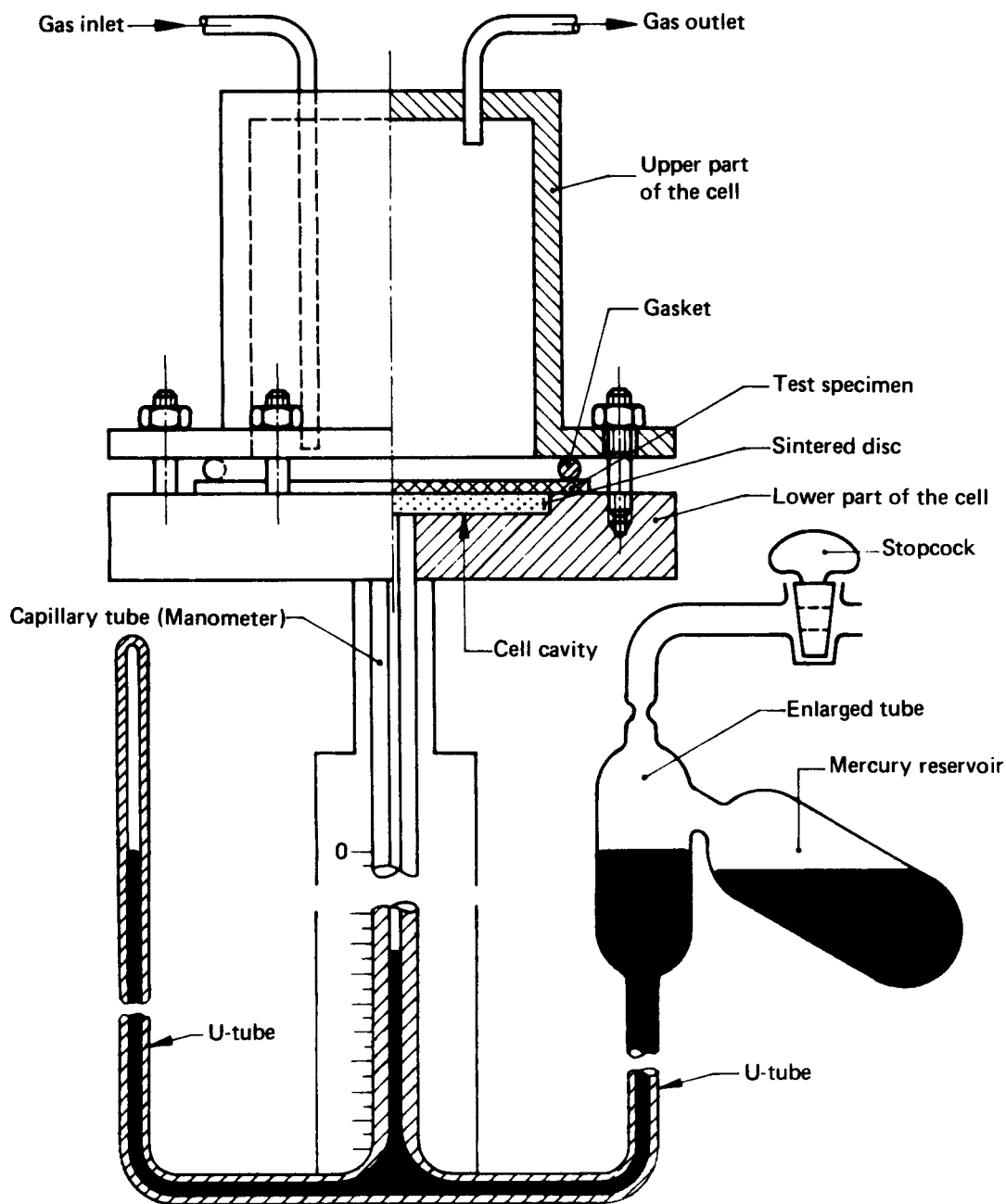
Figure 2 — Example of apparatus without overflowing [5.4, 2]
