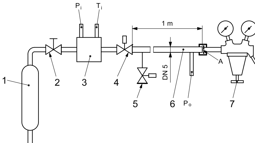
Figure 8 — Example of test apparatus for the external leakage test
