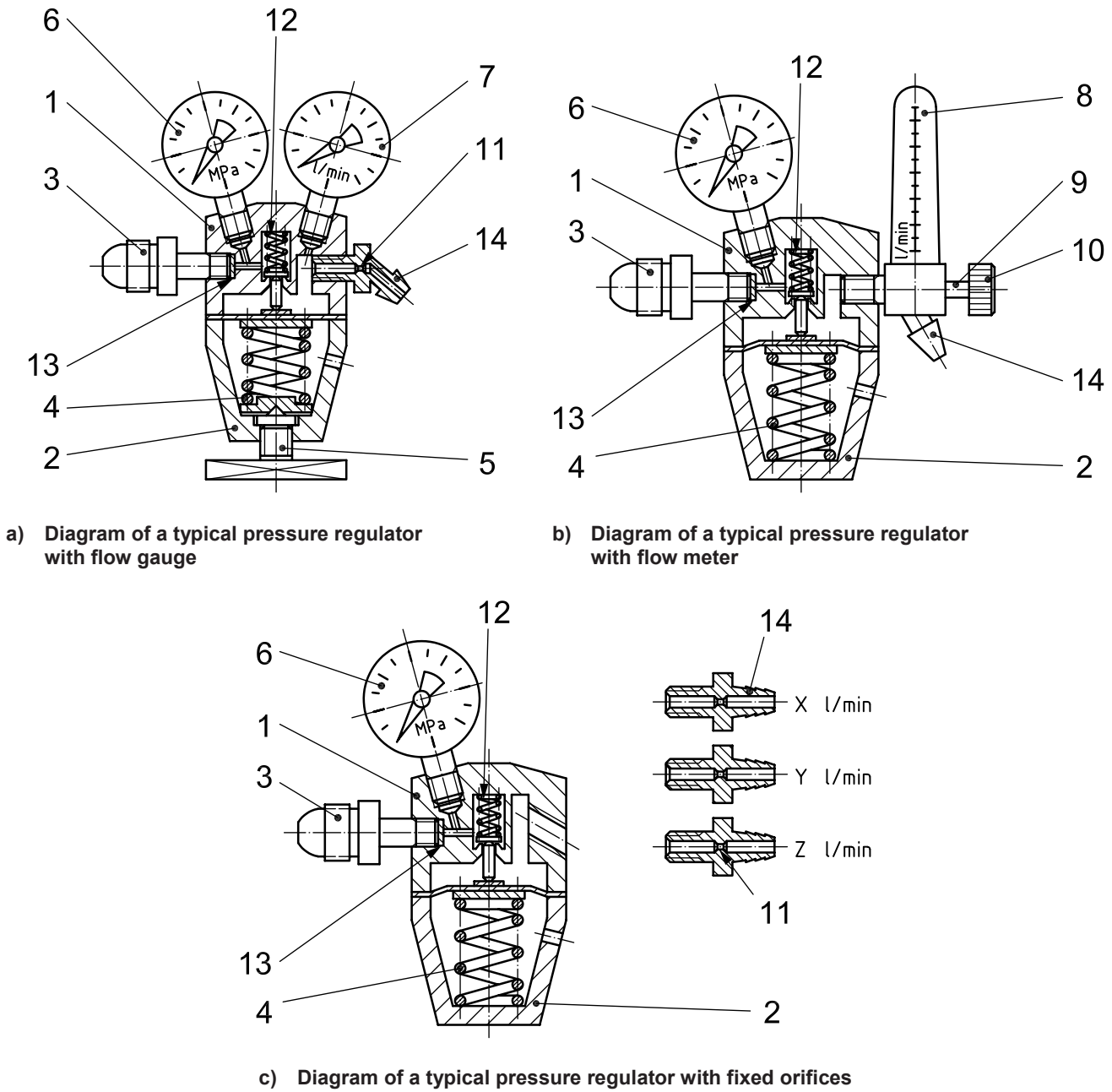
Figure A.2 — Typical pressure regulators
