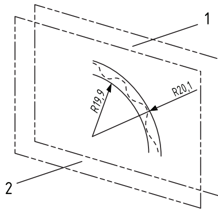
c) Tolerance zone
