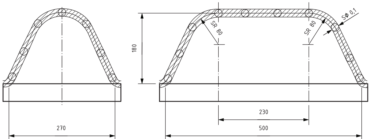
b) Interpretation (obsolete)
