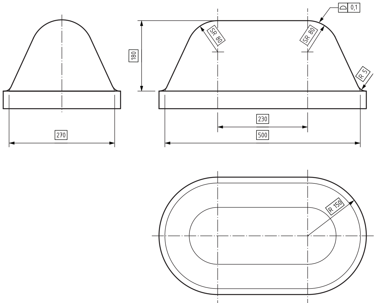
a) Indication on the drawing
