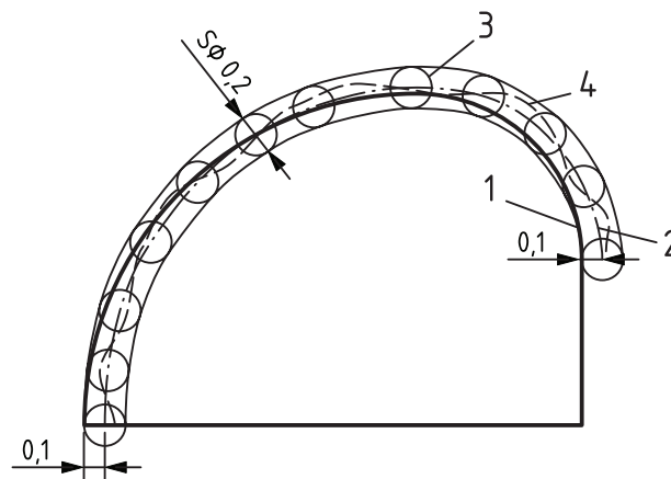
c) Tolerance zone
