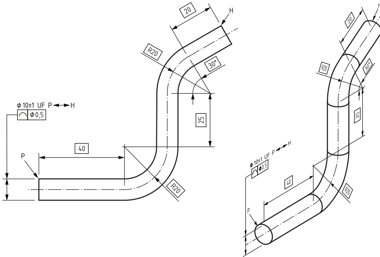
a) 2D drawing indication
