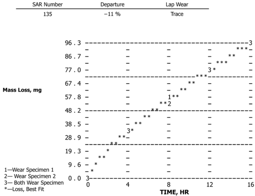
FIG. X1.7 Slurry Abrasion Response (SAR Number) Determination by Miller Number System—Test RS-1
