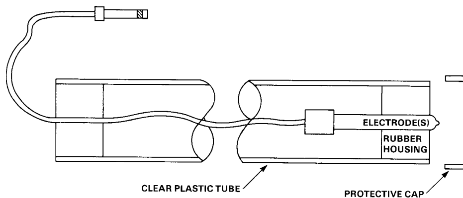
FIG. 1 Subsurface Probe
