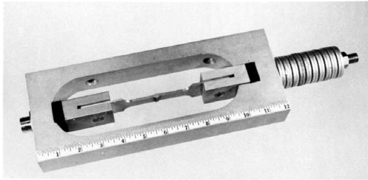
FIG. 2 Spring-Loaded Stressing Frame (7)
