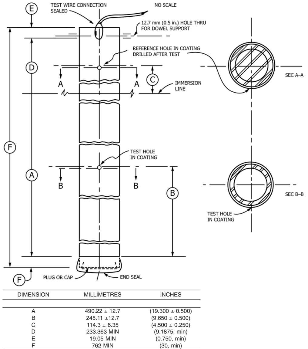
FIG. 3 Recommended Dimensions for Specimen
