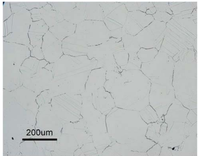
(l) Original with 200 Micron Bar, Rejectable
