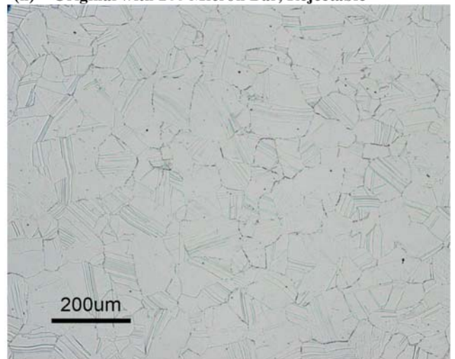
(p) Original with 200 Micron Bar, Rejectable
