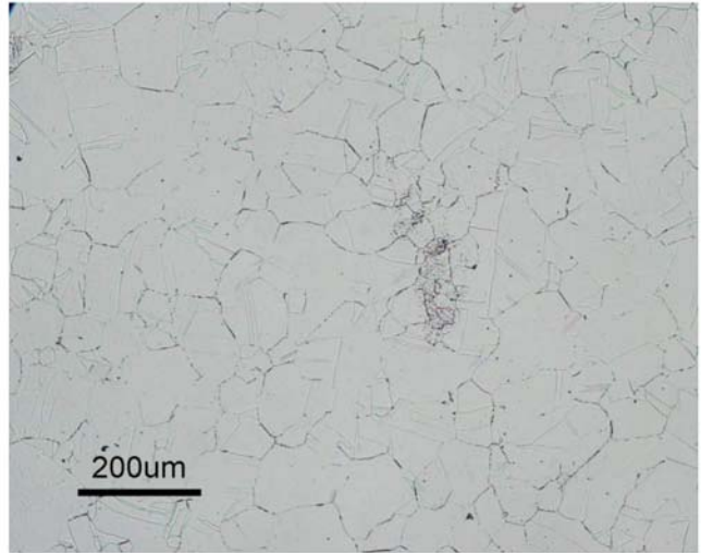
(t) Original with 200 Micron Bar, Rejectable
