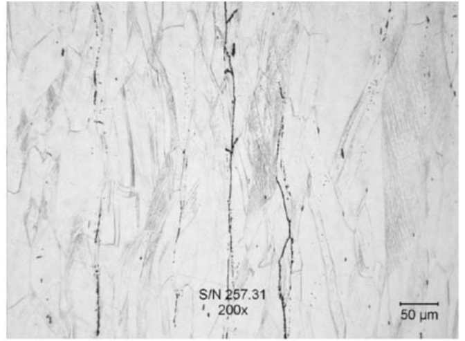
(h) 200X Original Magnification, Rejectable
