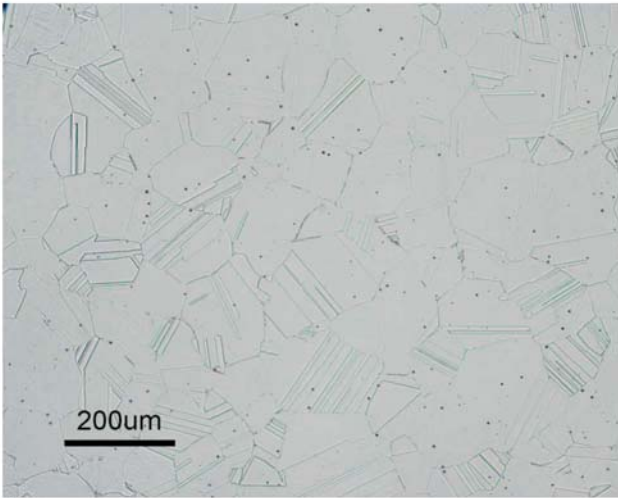
(o) Original with 200 Micron Bar, Acceptable
