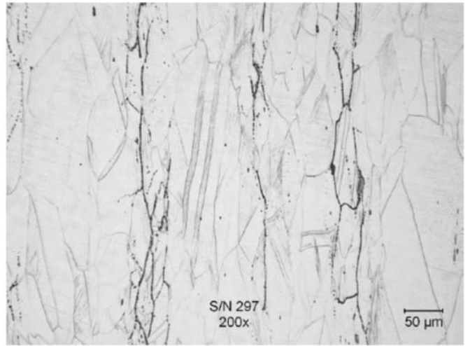
(j) 200X Original Magnification, Rejectable
