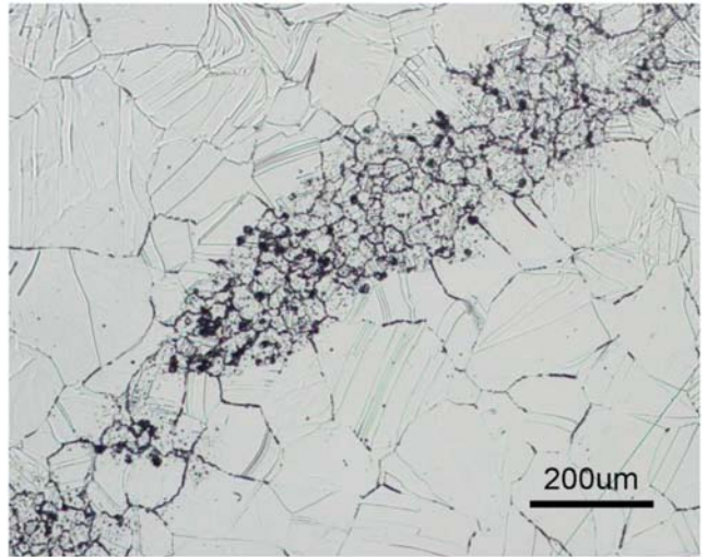
(n) Original with 200 Micron Bar, Rejectable
