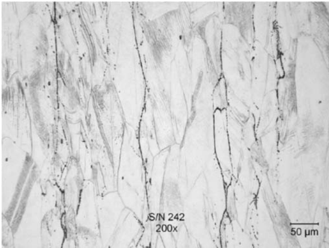
(g) 200X Original Magnification, Rejectable
