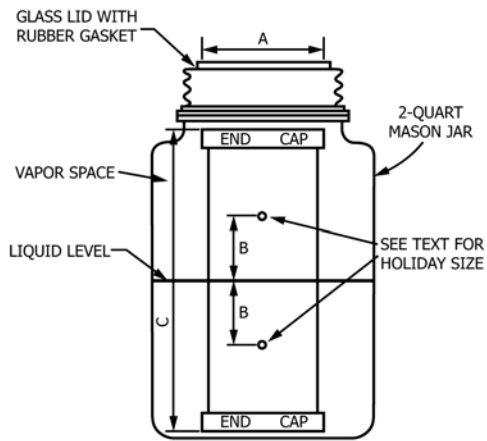
Dimensions A—70 mm (2.75 in.) Jar Opening B—45 mm (1.75 in.) Holiday Location C—90 mm (7.00 in.) Length of Pipe Specimen
