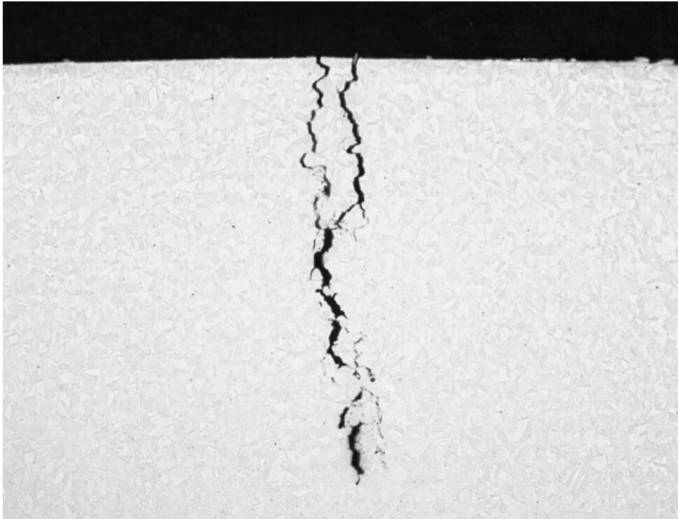
FIG. 7 Micrograph Showing Example of Intergranular SCC (Magnification 100x)
