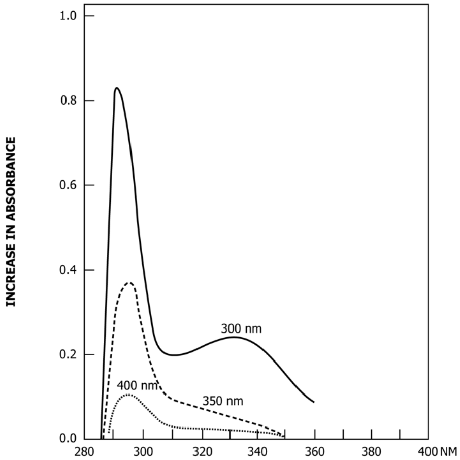
FIG. X1.5 Activation Spectrum of Increase in 300 nm, 350 nm, and 400 nm Absorbance of a Polycarbonate Film Exposed to Xenon Arc Radiation Through Daylight Type Filters Spectrally Separated by a Quartz Prism Spectrograph
