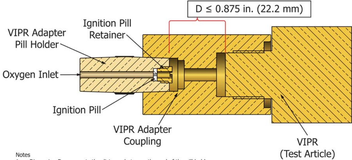
FIG. 20 Typical Ignition Pill Installed in VIPR Adapter Block
