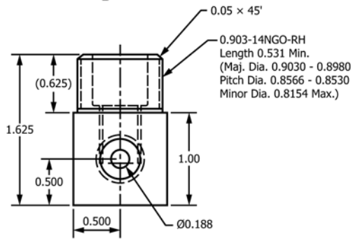
FIG. 10 CGA 540 Adapter Block
