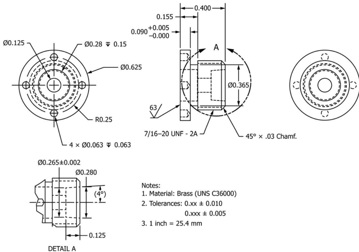
FIG. 13 CGA 870 Adapter Pill Holder
