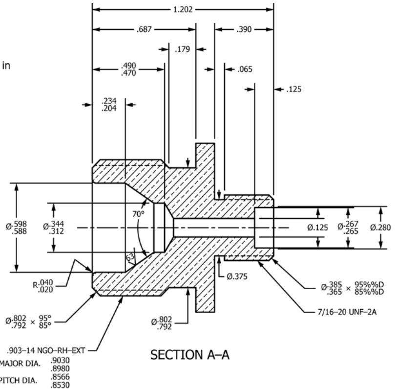
FIG. X4.2 CGA 540 Adapter Block (alternative)
