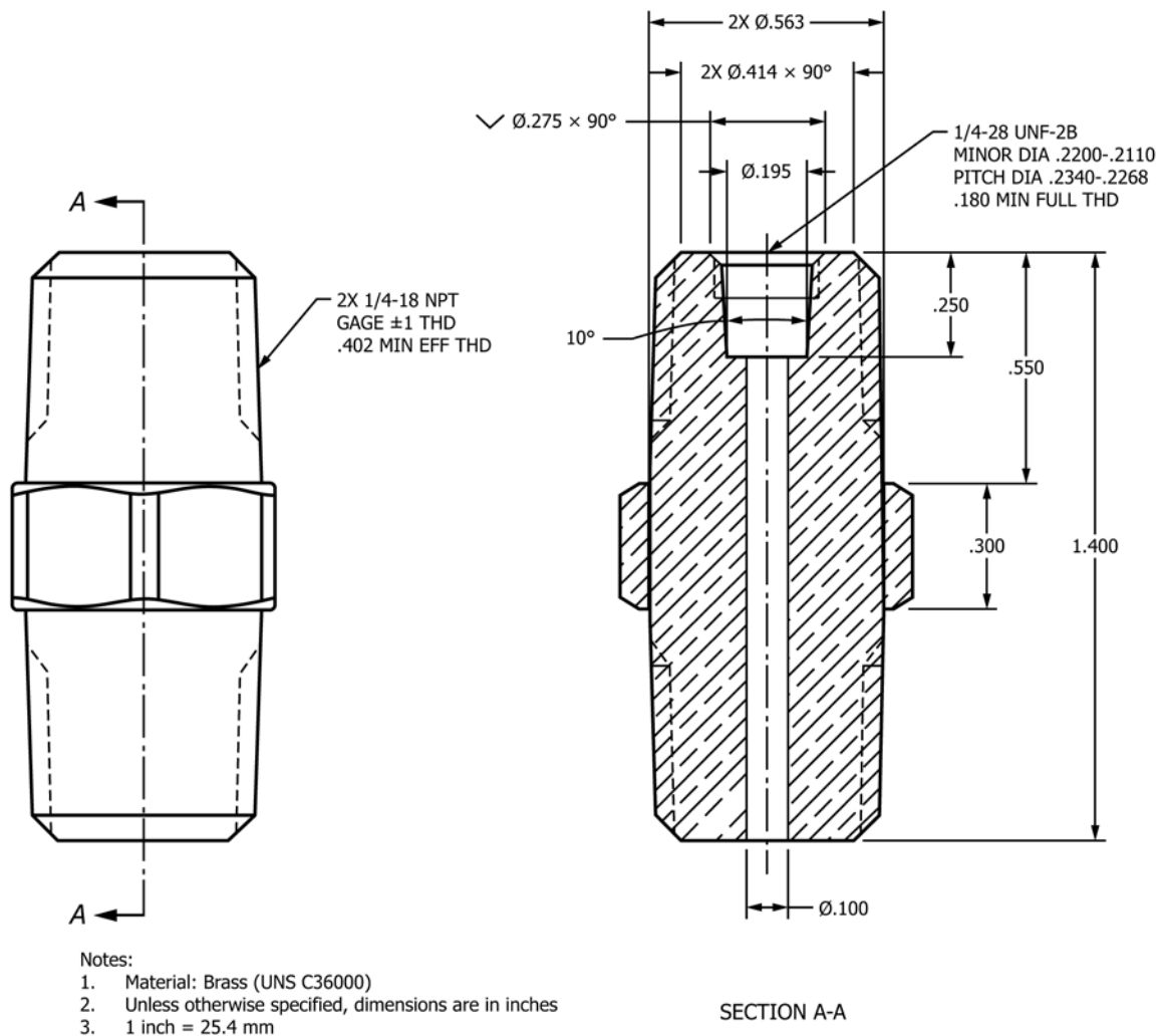
FIG. 16 VIPR Adapter Pill Holder
