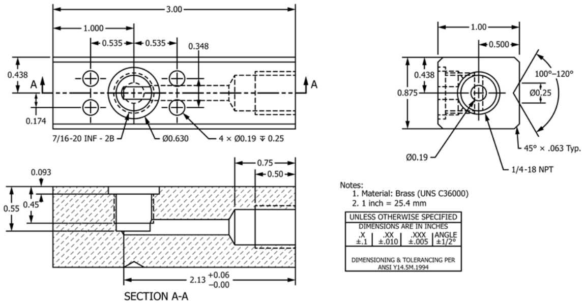
FIG. 12 CGA 870 Adapter Block
