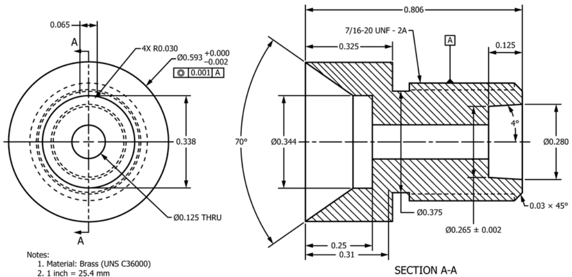
FIG. 10 CGA 540 Adapter Block
